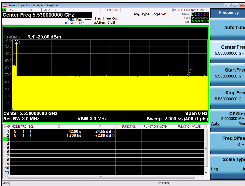
Test Bandwidth / Channel : 80MHz / 5530 MHz
