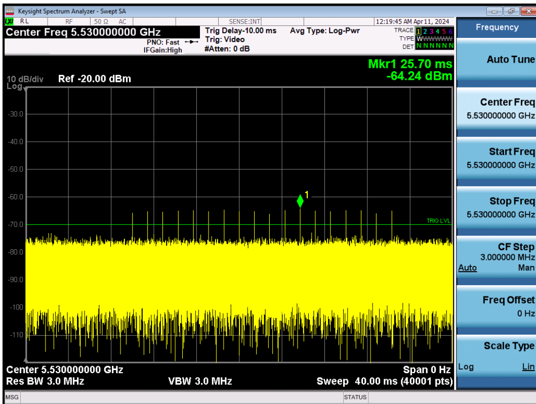
Test Bandwidth / Channel : 80MHz / 5530 MHz
