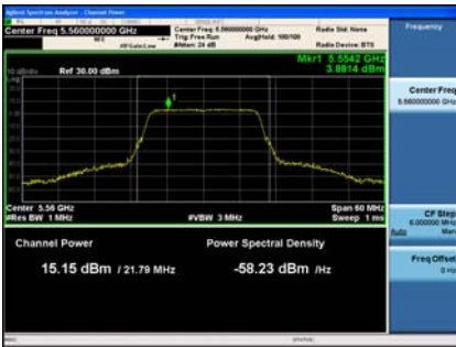
Antenna C
