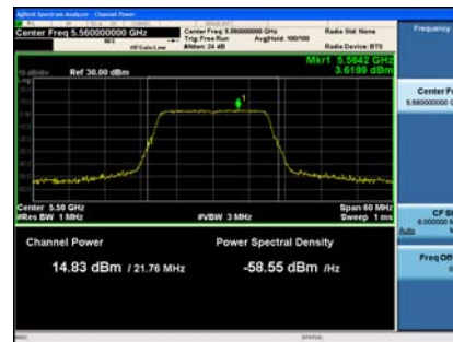
Antenna D
