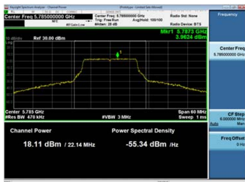
Antenna C
