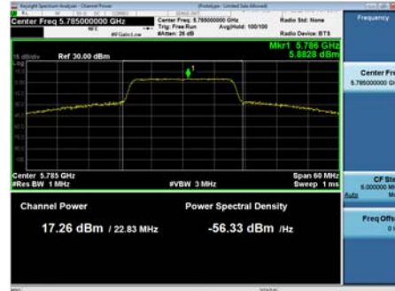
Antenna B
