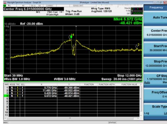
Antenna B
