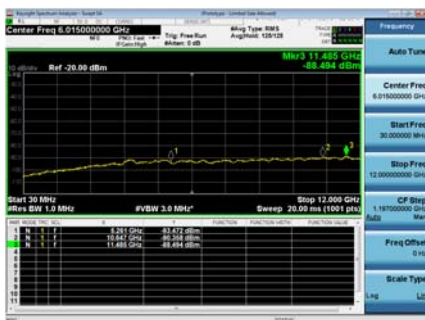
Antenna C
