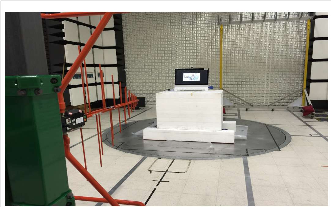
Title: Radiated Emissions Below 1 GHz
