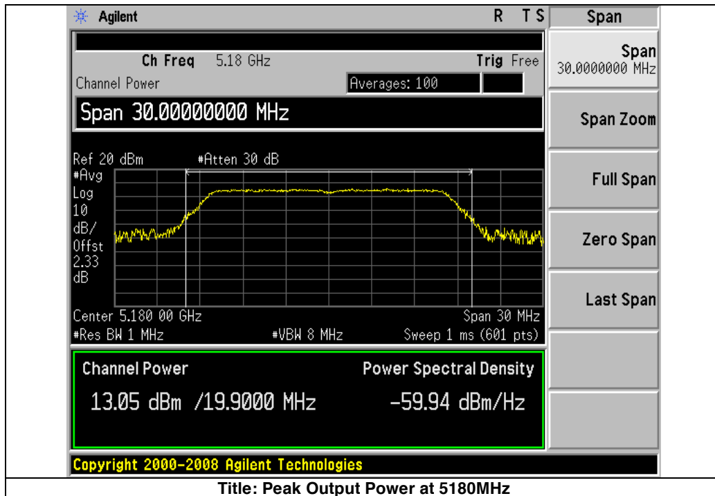
Title: Peak Output Power at 5180MHz
