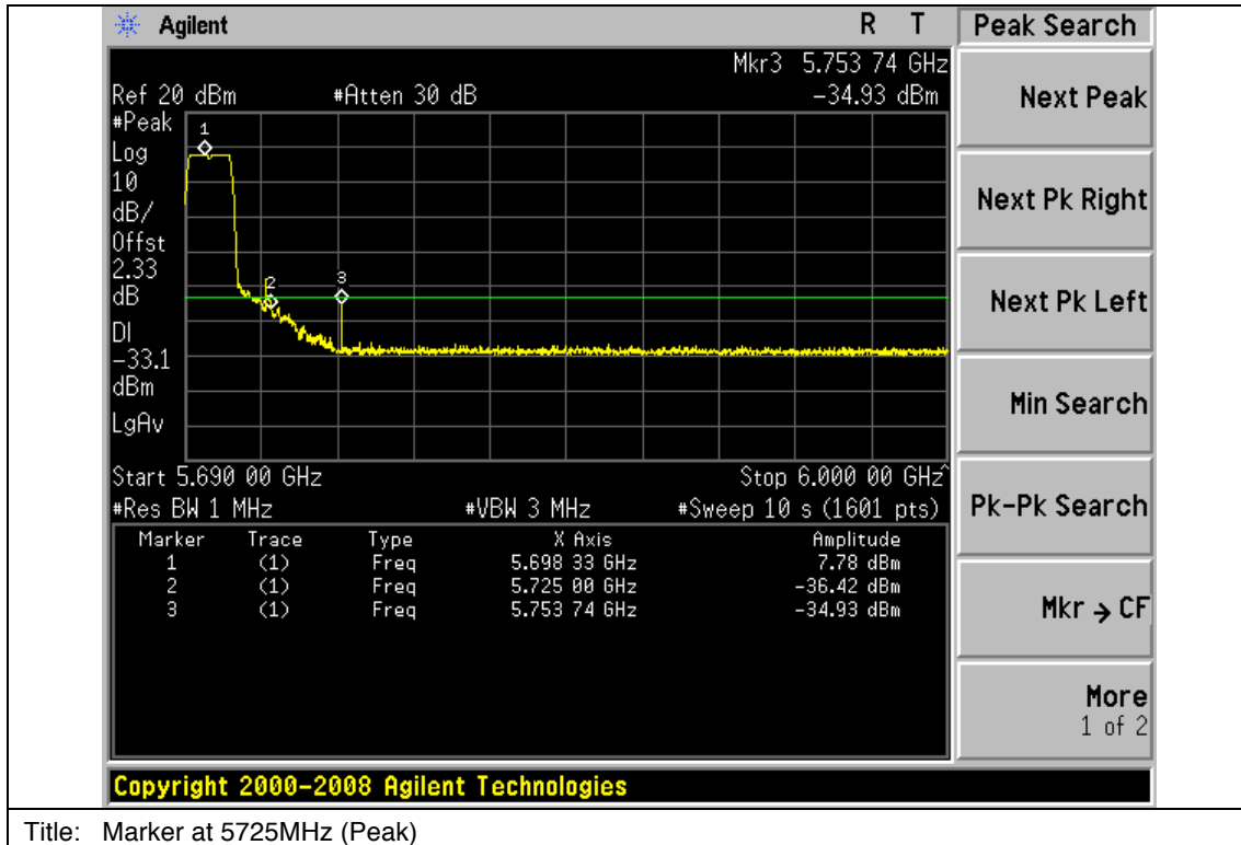
Title: Marker at 5725MHz (Peak)
