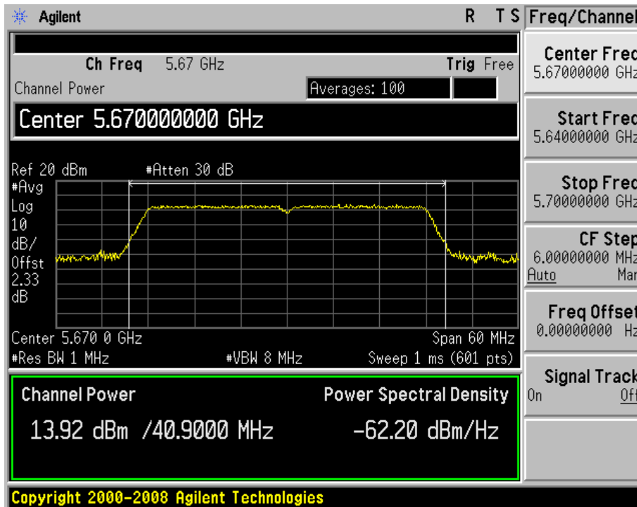
Graphical Test Results for Power Spectral Density for 802.11n (HT40):
