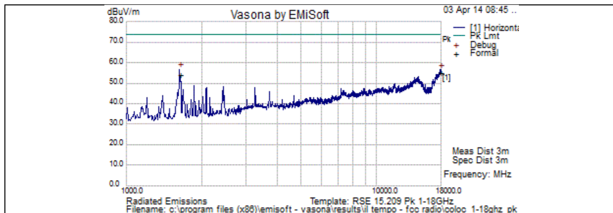
Title: Co-Location Radiated Spurious Emissions Results for 802.11b & Bluetooth: 1-18GHz (Peak)
