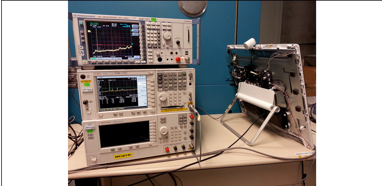
Title: Conducted Spurious Emissions Test Configuration
