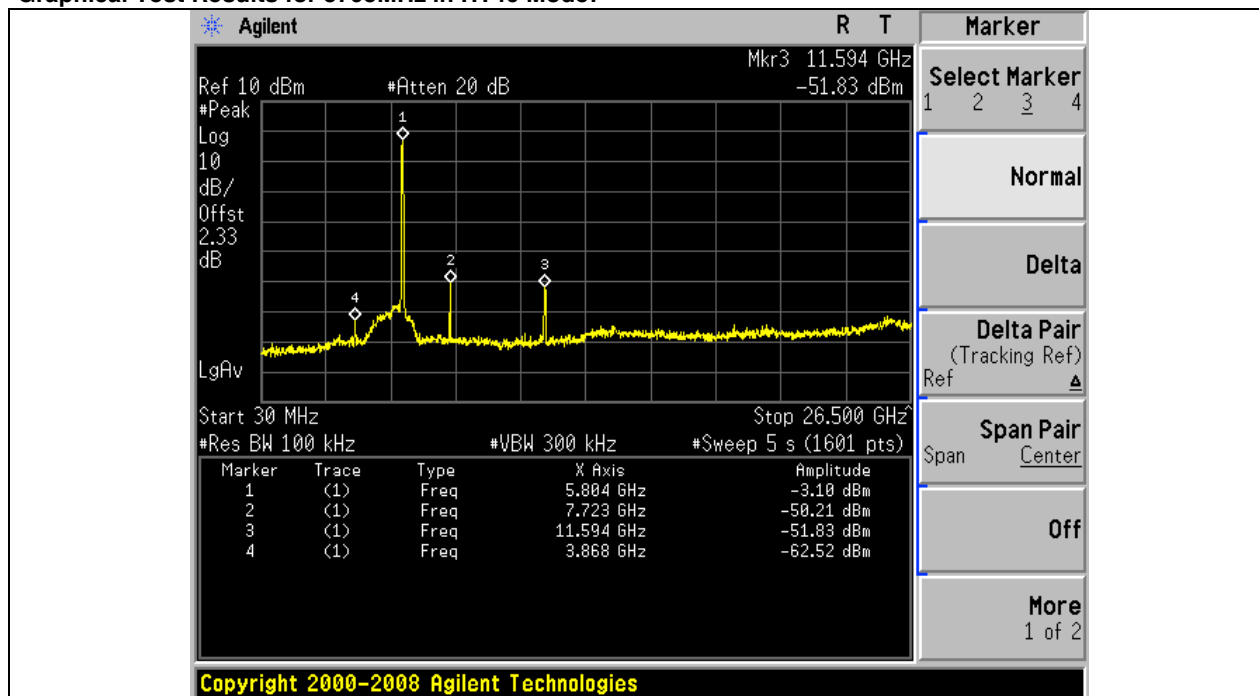
Title: 30dBc Conducted Spurious Emissions – 802.11nHT40 - 5795MHz
