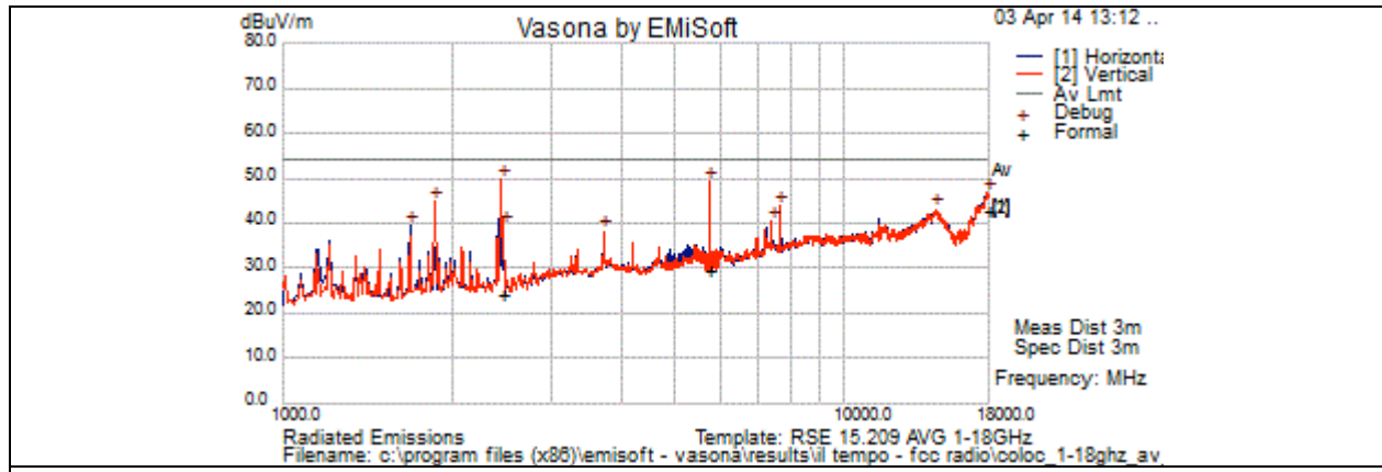
Title: 1 - 18GHz Test Results for HT40 & Bluetooth (Average)
