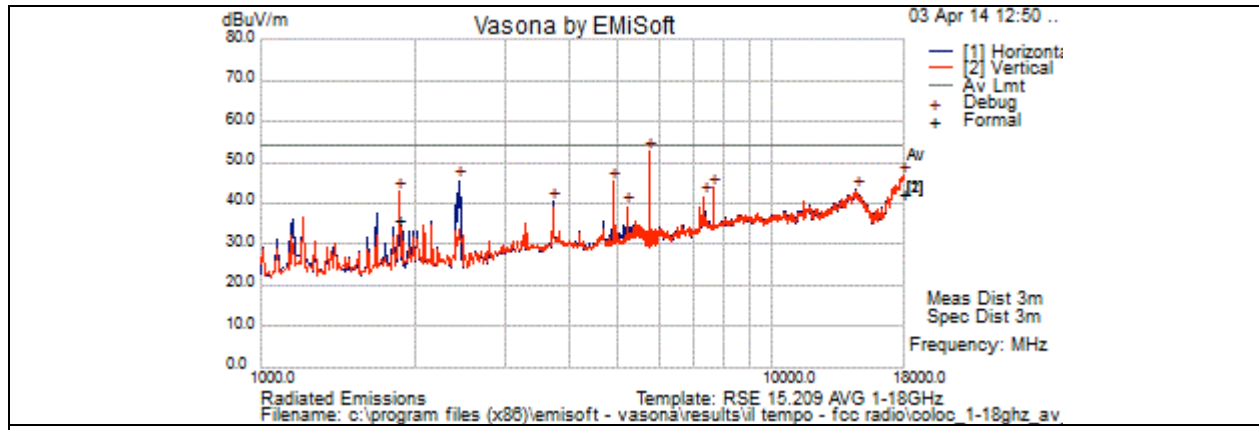
Title: 1 - 18GHz Test Results for HT20 & Bluetooth (Average)
