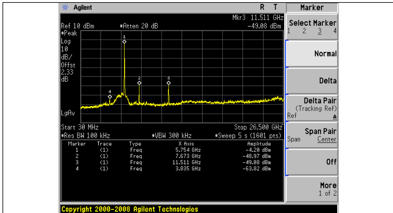
Title: 30dBc Conducted Spurious Emissions – 802.11nHT40 - 5755MHz
