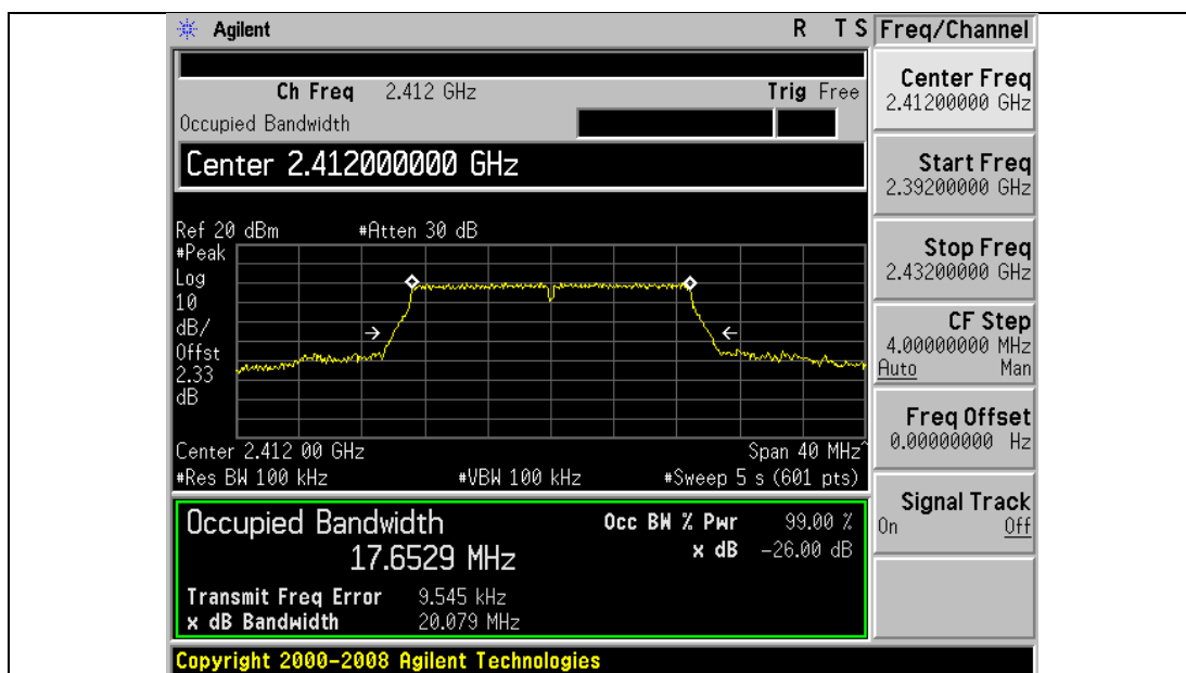
Title: Occupied Bandwidth 2412MHz at M3 (802.11n HT20)
