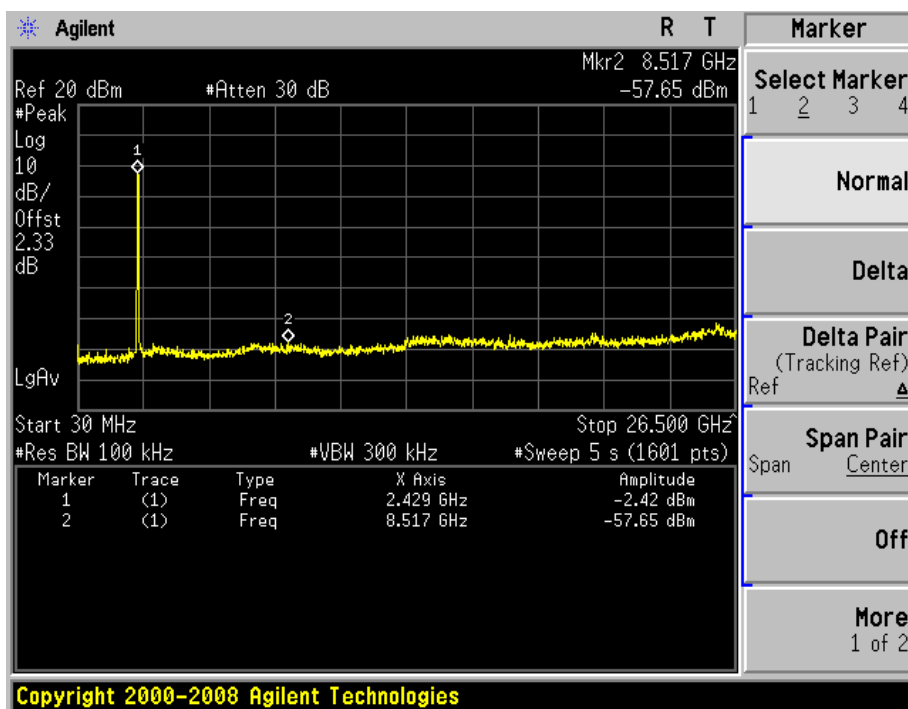
Conducted Spurious Emissions – 802.11n HT40 (2442MHz)
