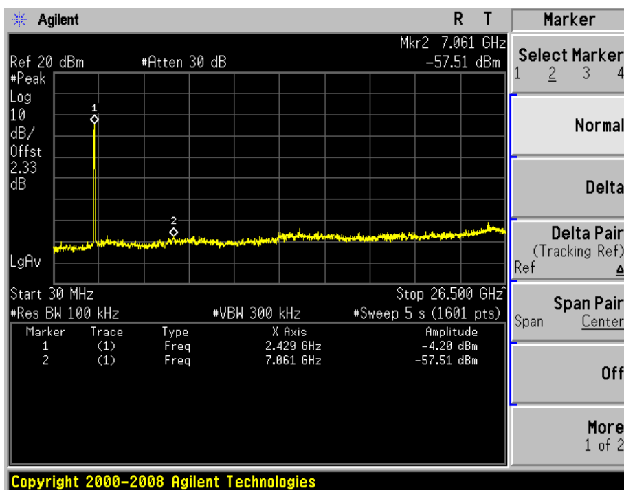
Conducted Spurious Emissions – 802.11n HT40 (2422MHz)
