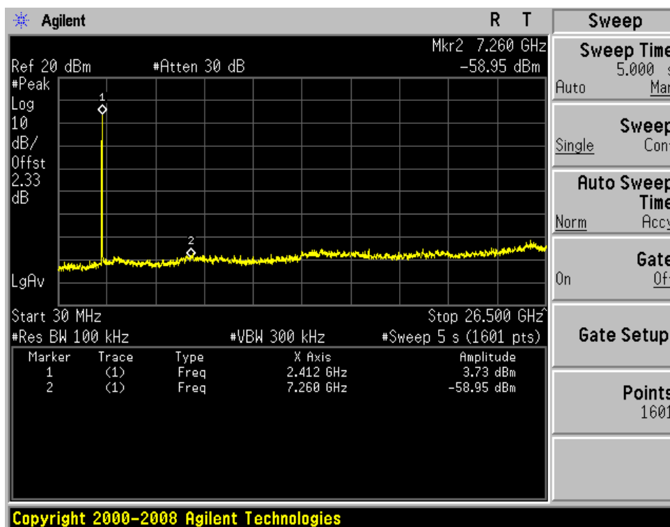
Conducted Spurious Emissions – 802.11b (2412MHz)
