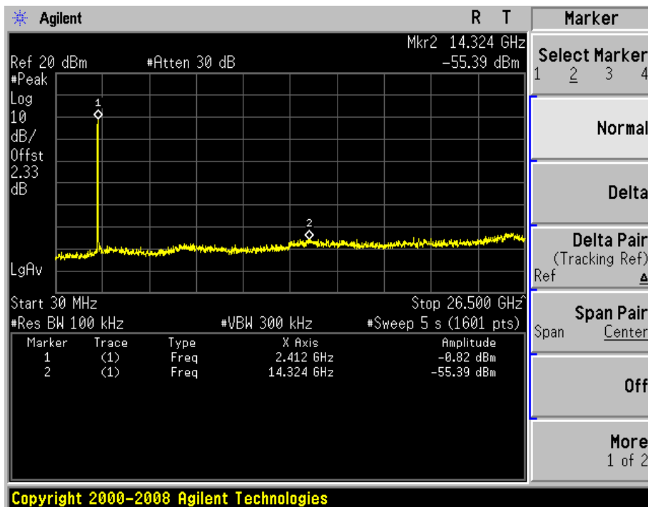
Conducted Spurious Emissions – 802.11g (2412MHz)
