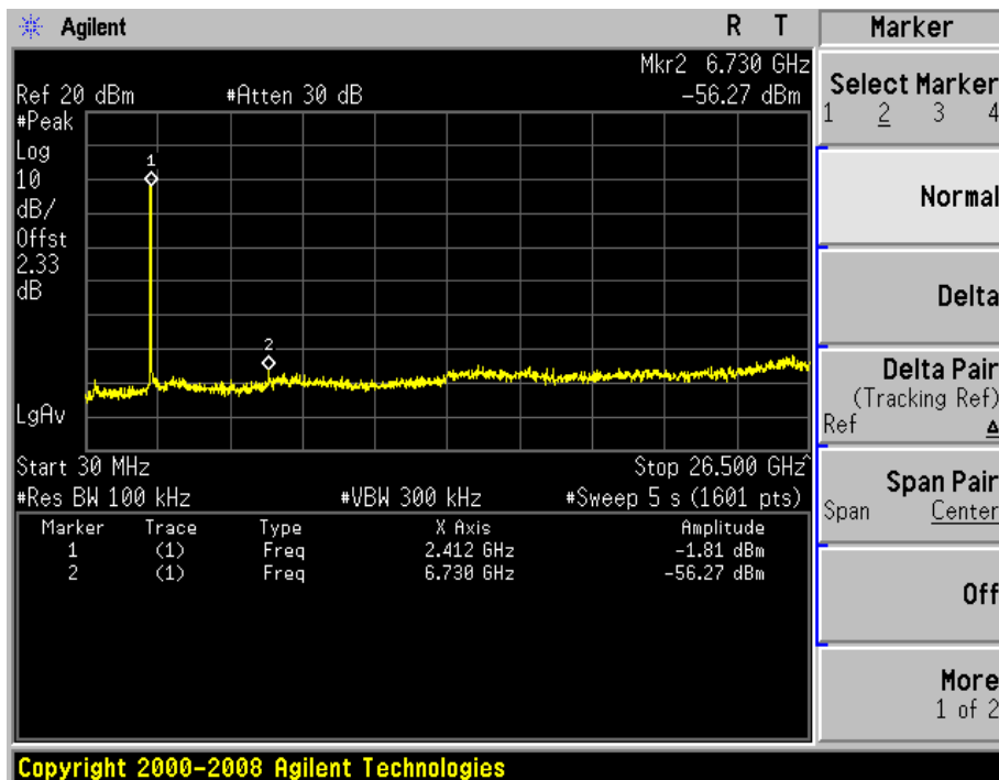
Conducted Spurious Emissions – 802.11n HT20 (2412MHz)
