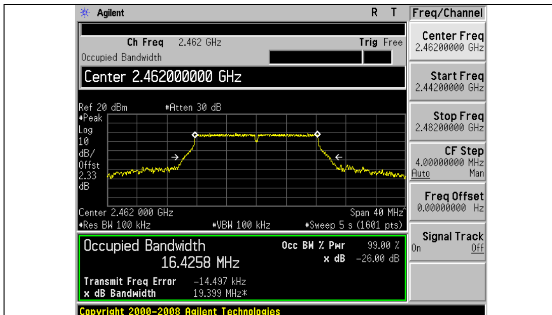
Title: Occupied Bandwidth 2462MHz at 6Mbps (802.11g)
