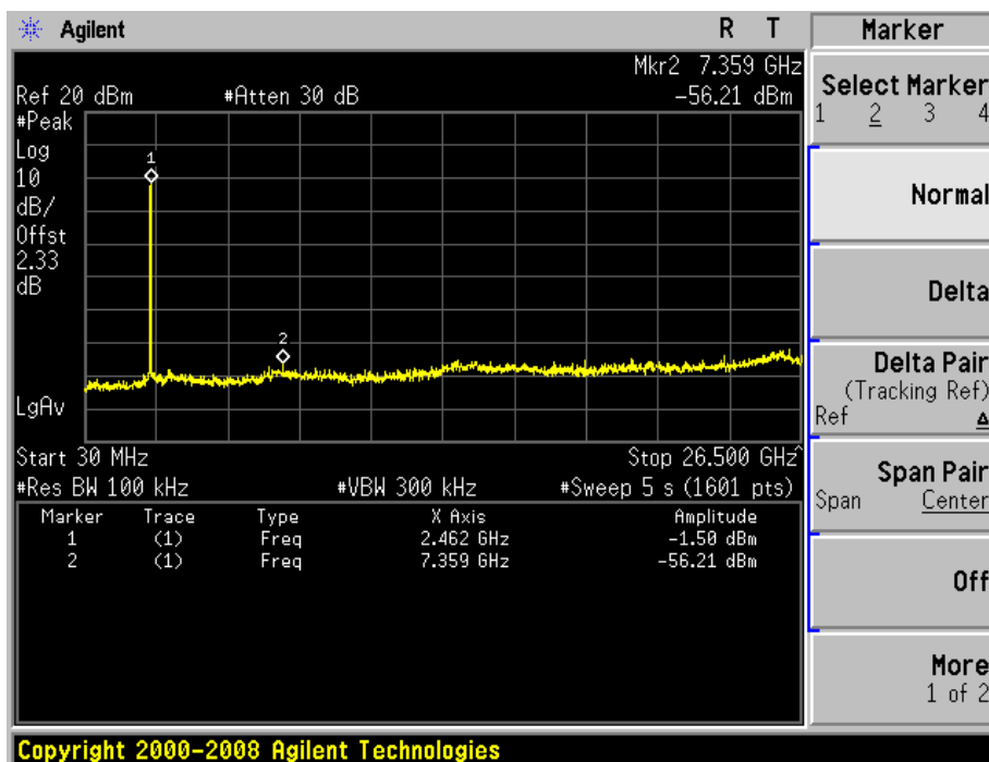
Conducted Spurious Emissions – 802.11n HT20 (2462MHz)
