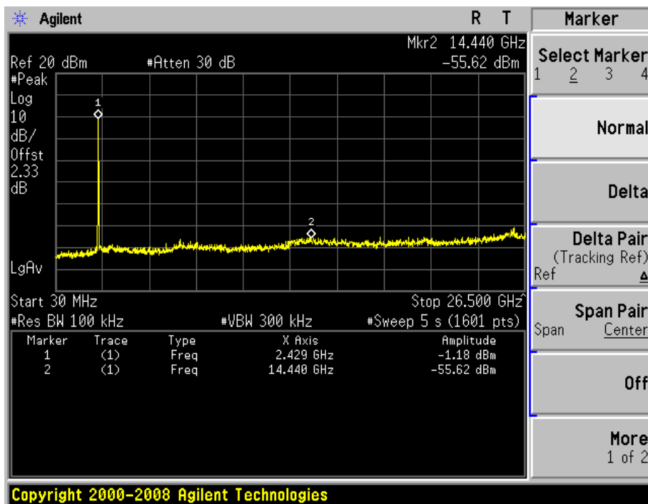
Conducted Spurious Emissions – 802.11g (2437MHz)
