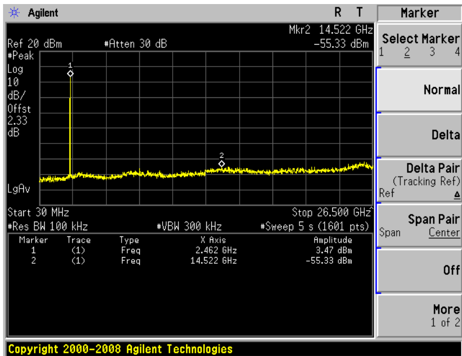
Conducted Spurious Emissions – 802.11b (2462MHz)
