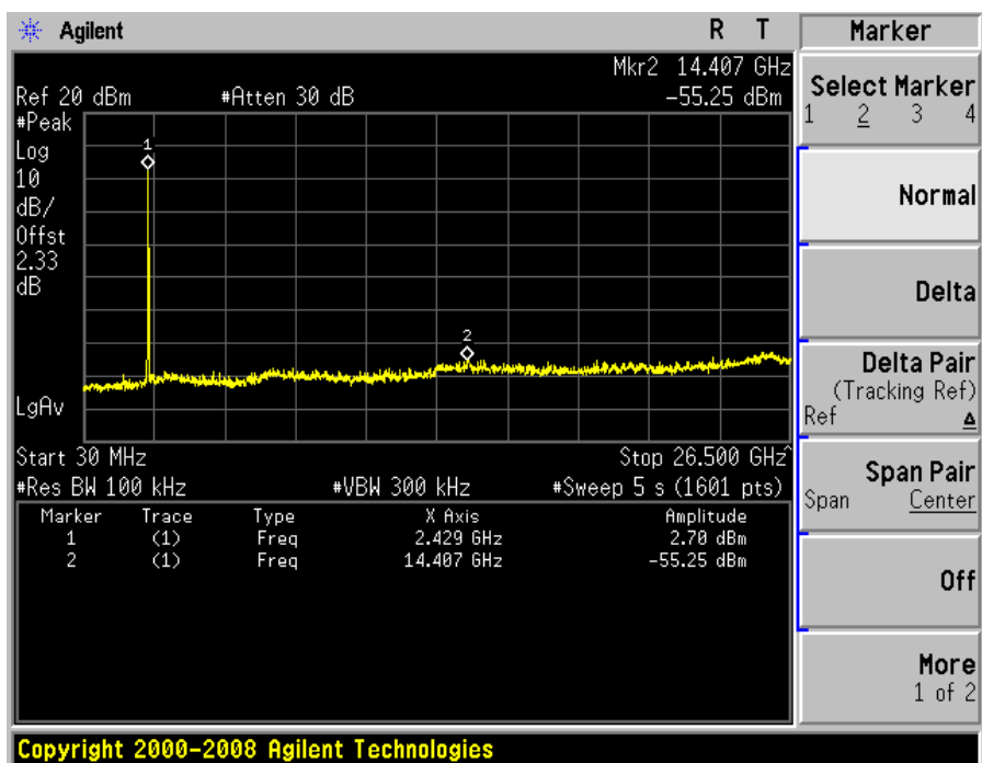
Conducted Spurious Emissions – 802.11b (2437MHz)
