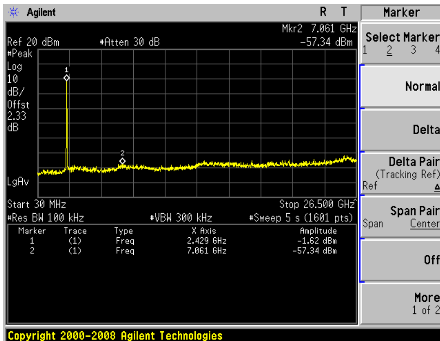
Conducted Spurious Emissions – 802.11n HT20 (2437MHz)
