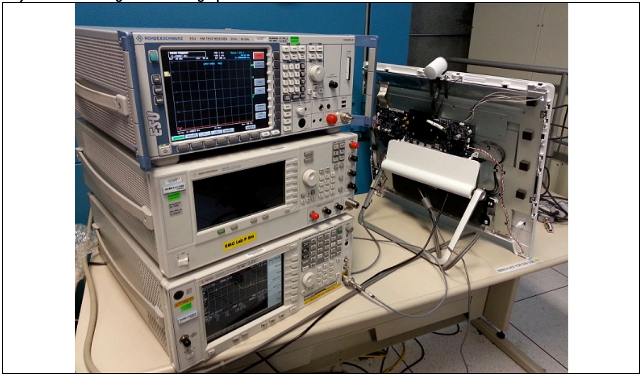
Title: Conducted Spurious Emissions - Test Setup
