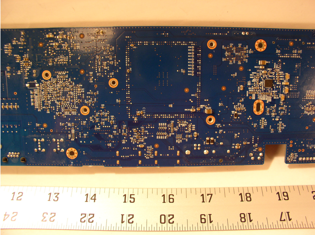
CP-DX80 : Internal PCB Mother Board (bottom 2/3) Close up view
