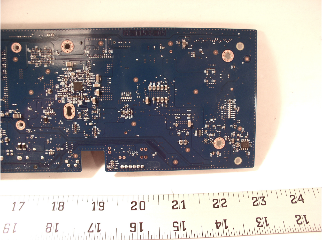
CP-DX80 : Internal PCB Mother Board (bottom 3/3) Close up view
