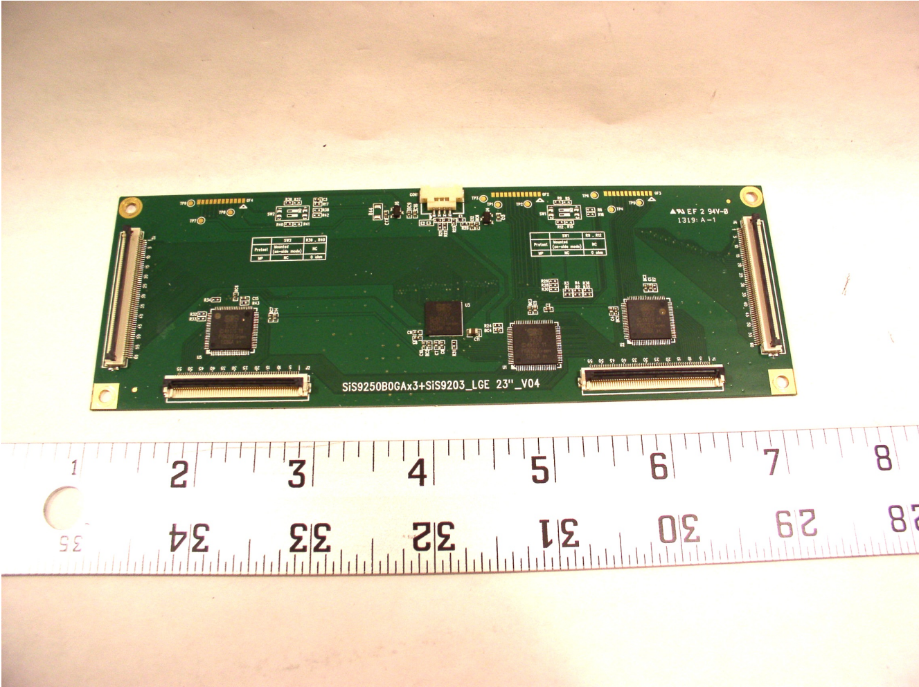
CP-DX80 : Internal PCB touch screen controller (Top view)
