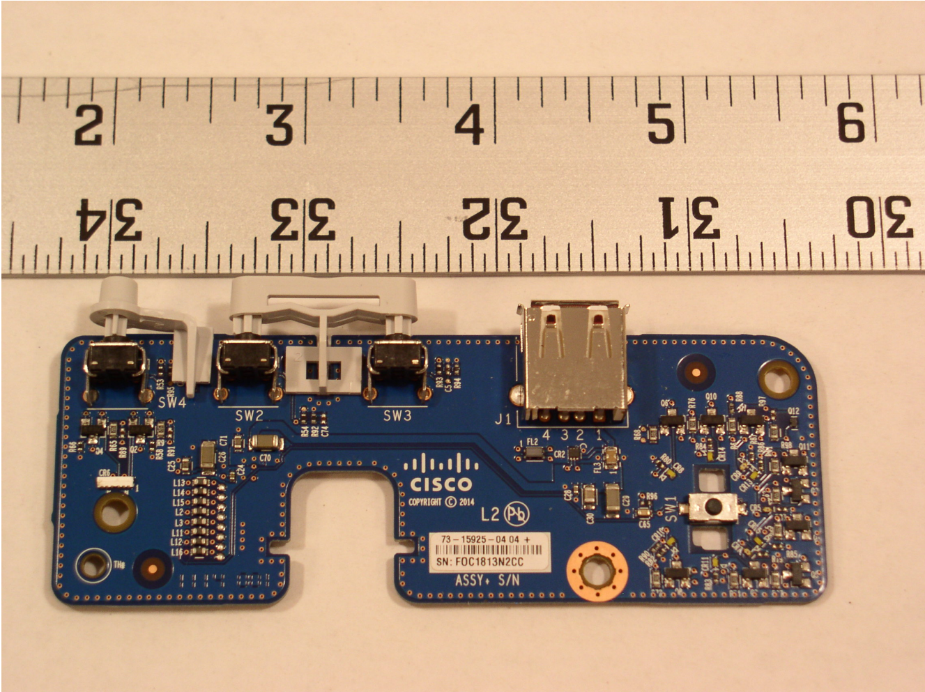
CP-DX80 : Internal PCB Volume and USB board (Top view)
