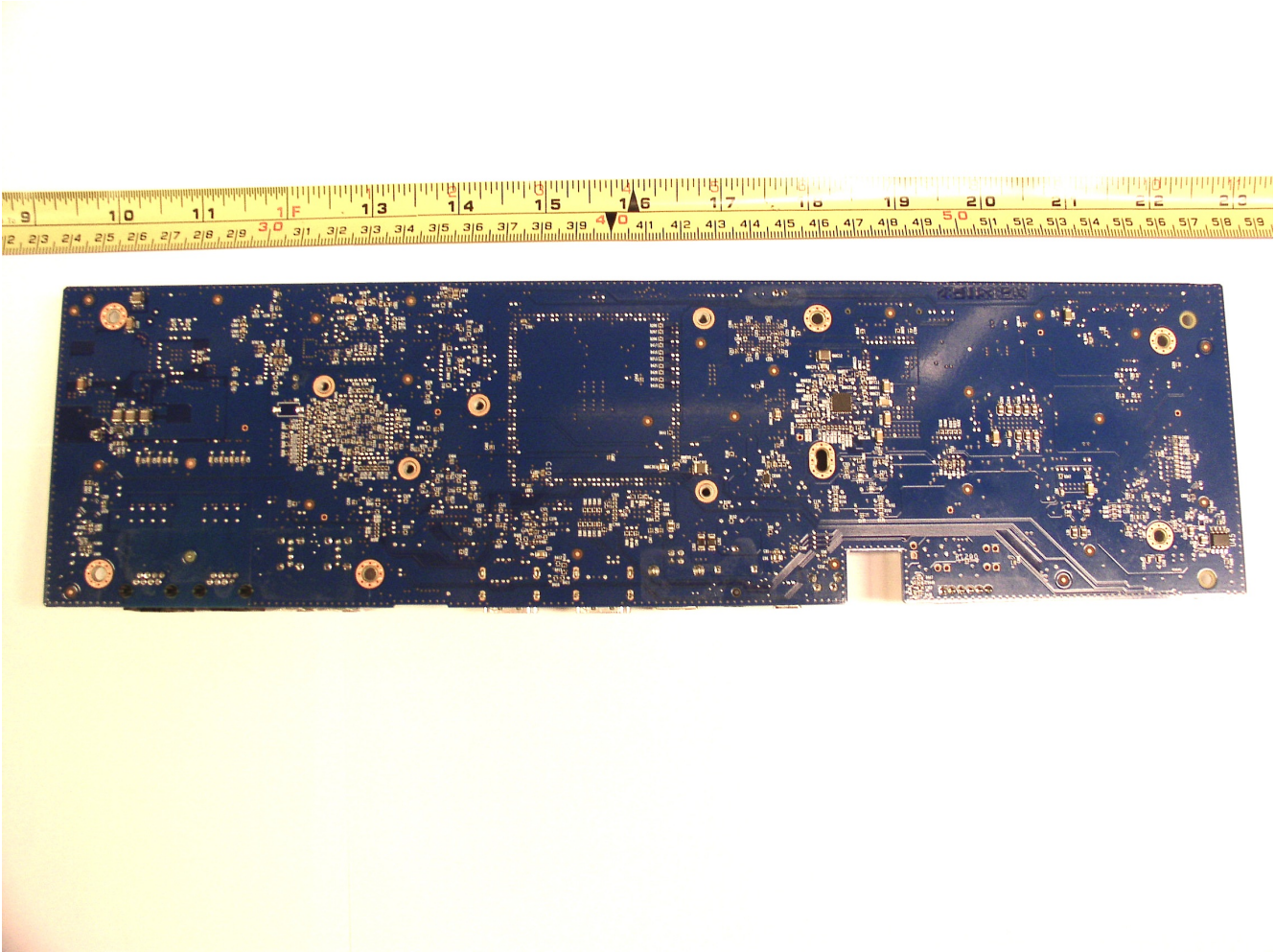
CP-DX80 : Internal PCB Mother Board (bottom view)
