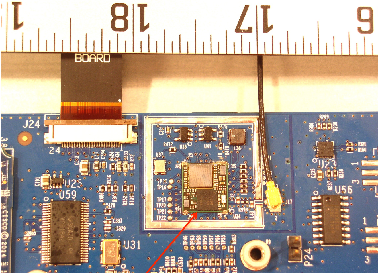
CP-DX80 : Internal PCB Mother Board (Radio Section with Shield removed)
