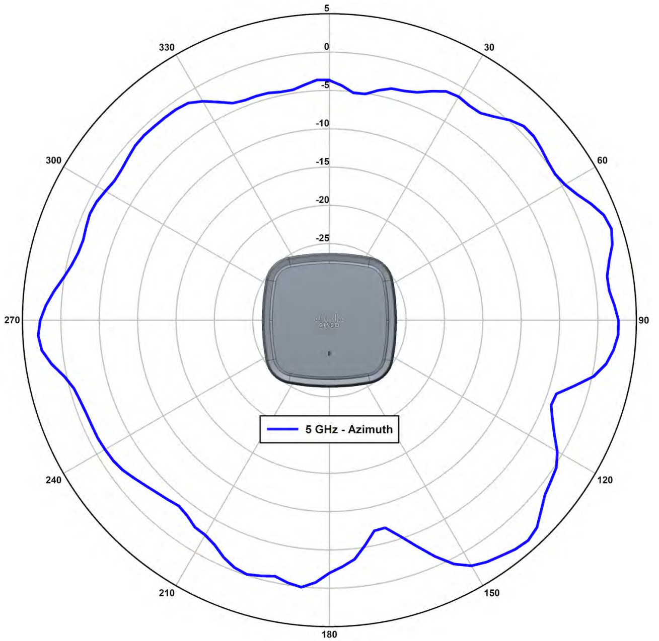
Figure 15 5 GHz - Azimuth - Port H
