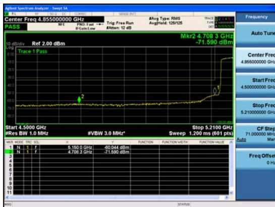
Antenna C
