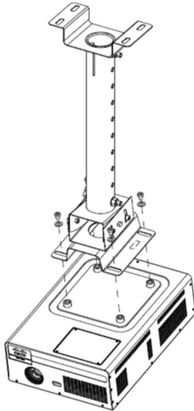
Figure 2-7 CEED 3700 Placement
