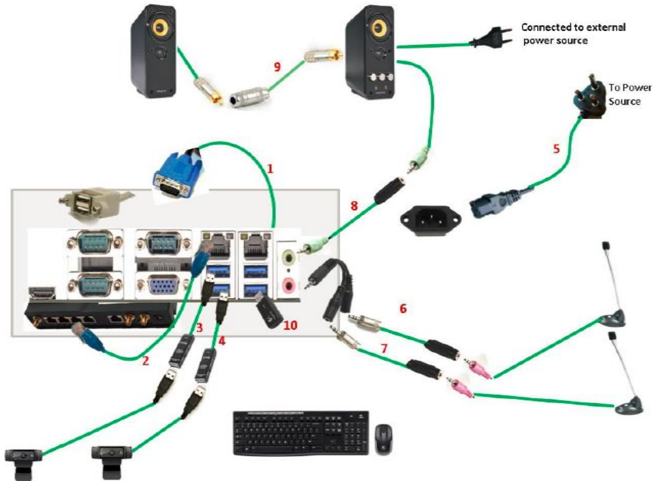
Figure 2-9 CEED 3700 External Cable Connections
