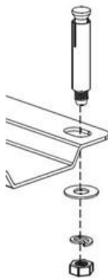
Figure 2-3 Fixing of the Anchor Bolts
