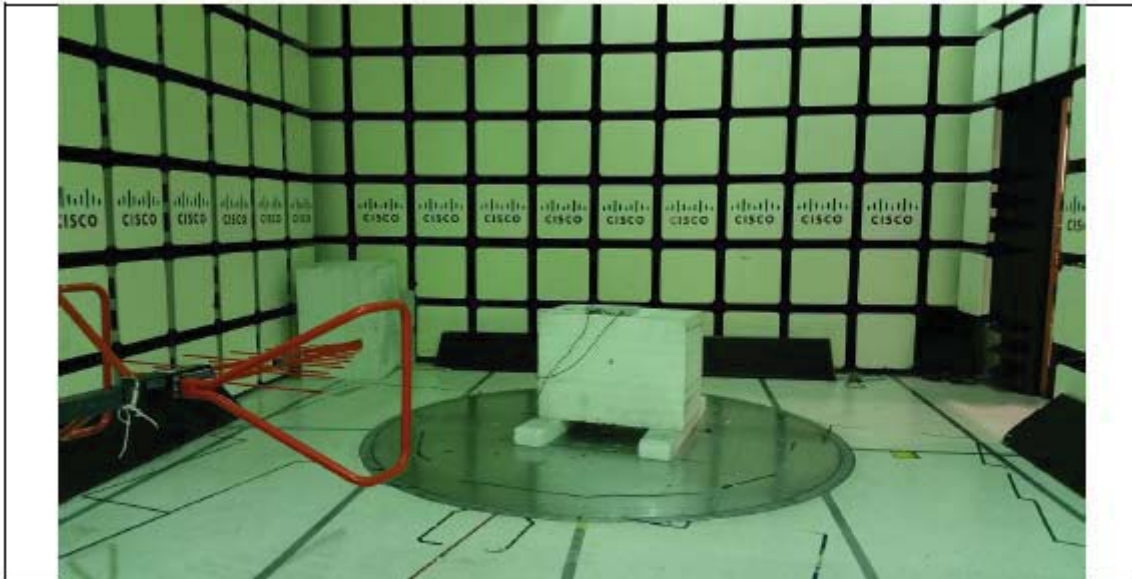
Title: Radiated Emissions Configuration Photograph 30MHz-1GHz
