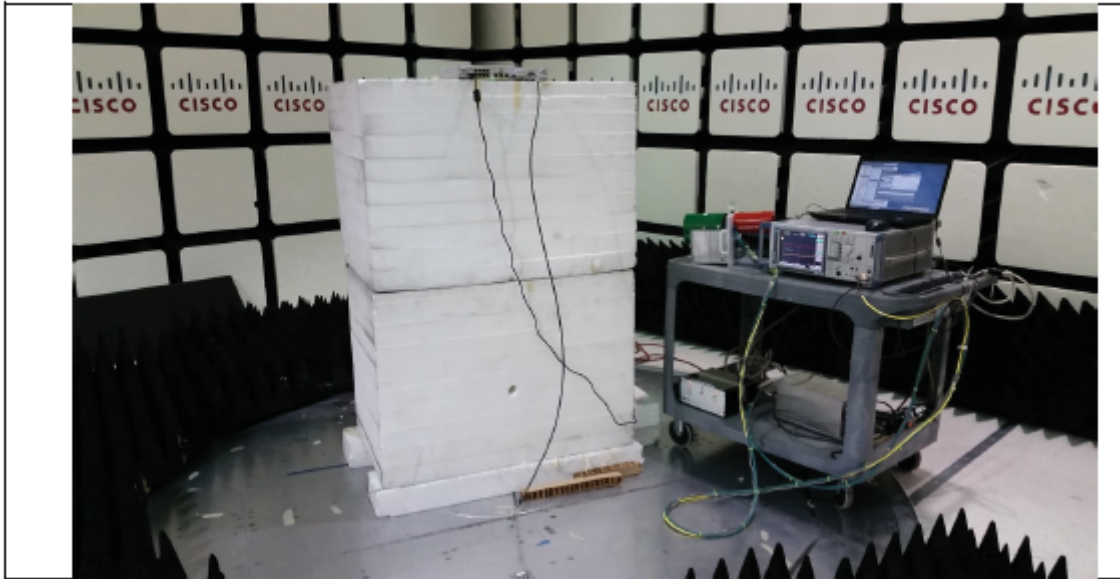
Title: Radiated Emissions Configuration Photograph 18-26.5GHz
