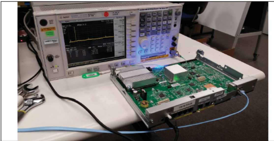
Title: Conducted Setup (Conducted Spurious Emissions)
