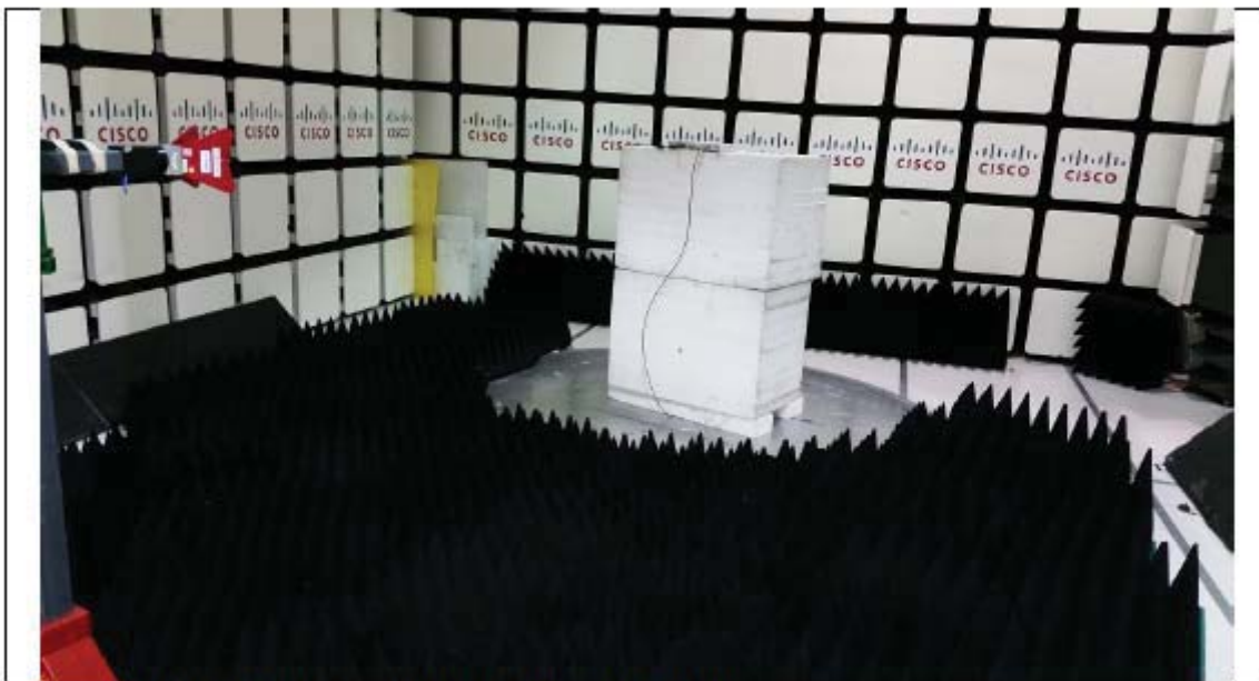
Title: Radiated Emissions Configuration Photograph 1-18GHz
