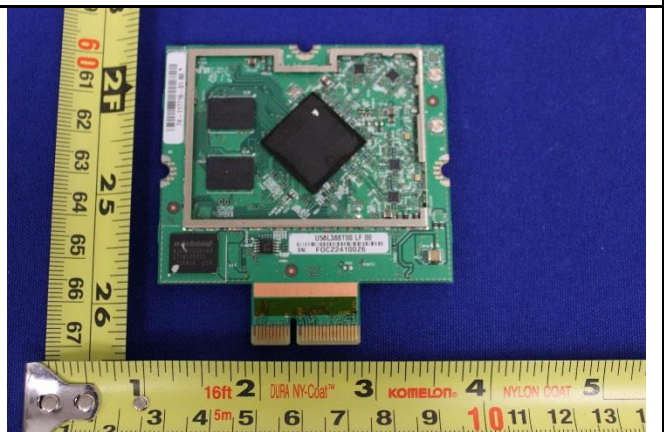
PCB2 Front Un-shielding cover View
