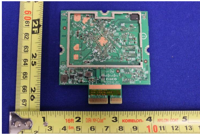
PCB2 Rear Un-shielding cover View
