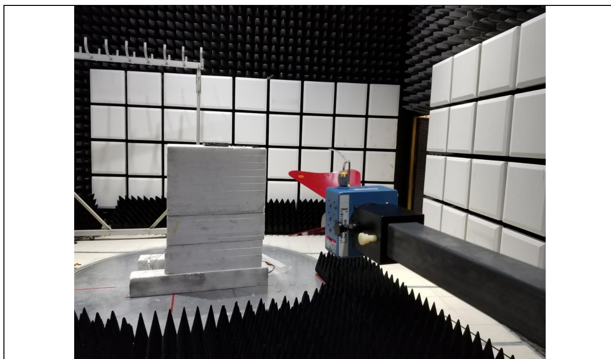
Title: Radiated Spurious Emissions Test Configuration 18 – 40GHz
