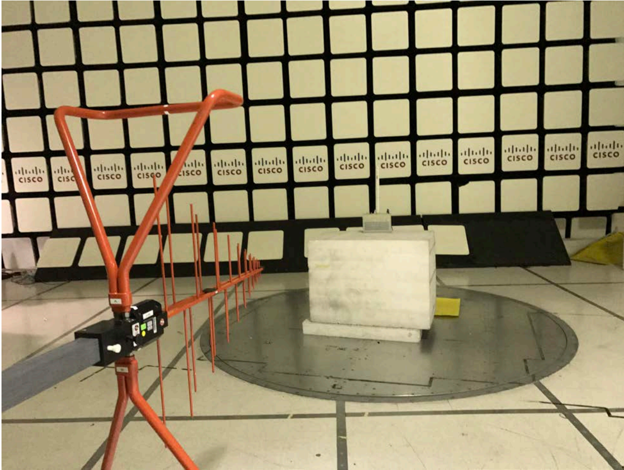
Radiated Emissions 30MHz-1GHz Configuration Photograph
