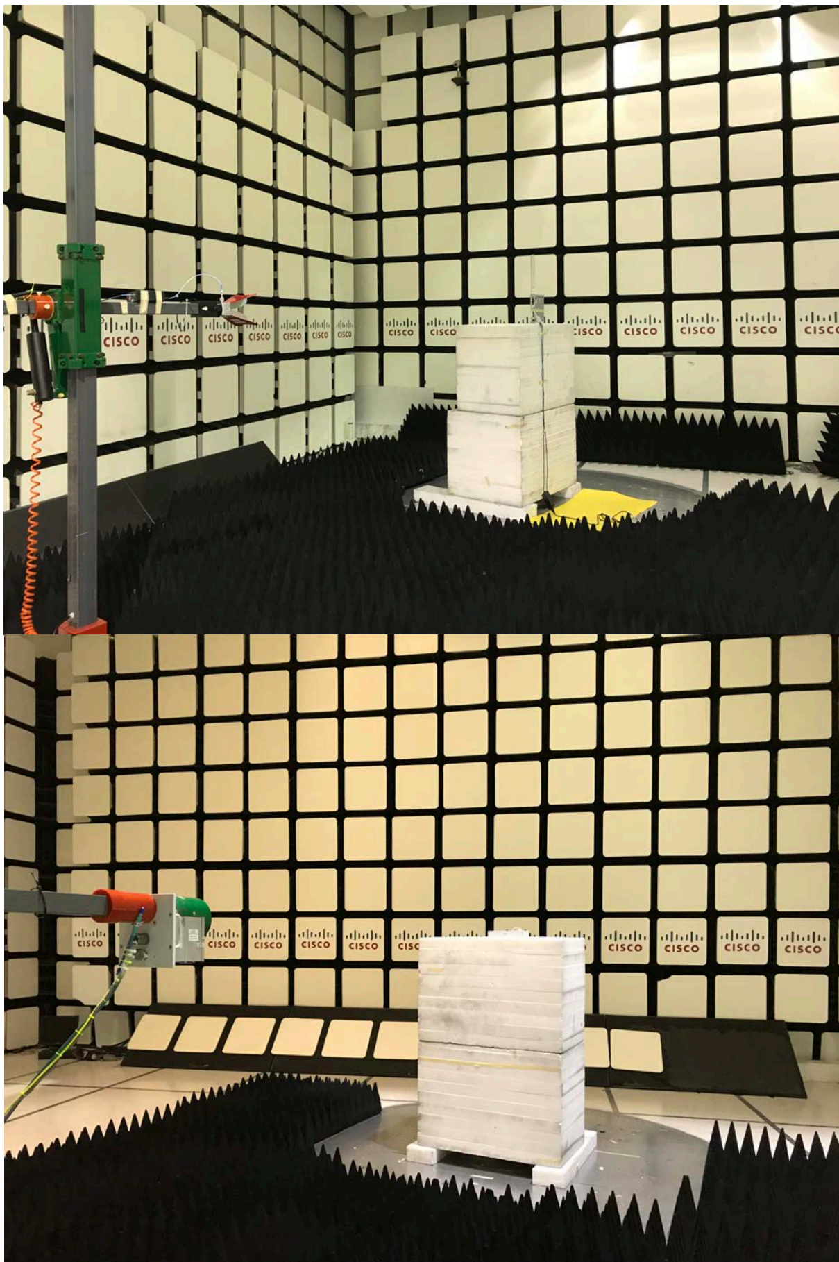
Radiated Emissions 1-18GHz Configuration Photograph
