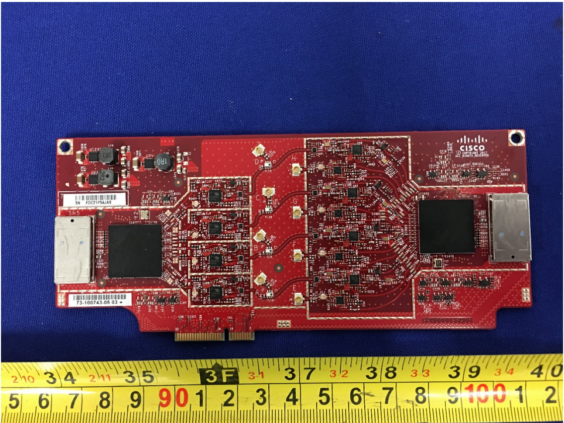
RF Board top side
