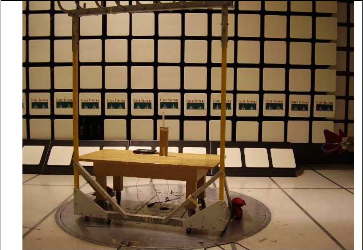
Title: Bandedge test for 7.5dbi Omni test setup
