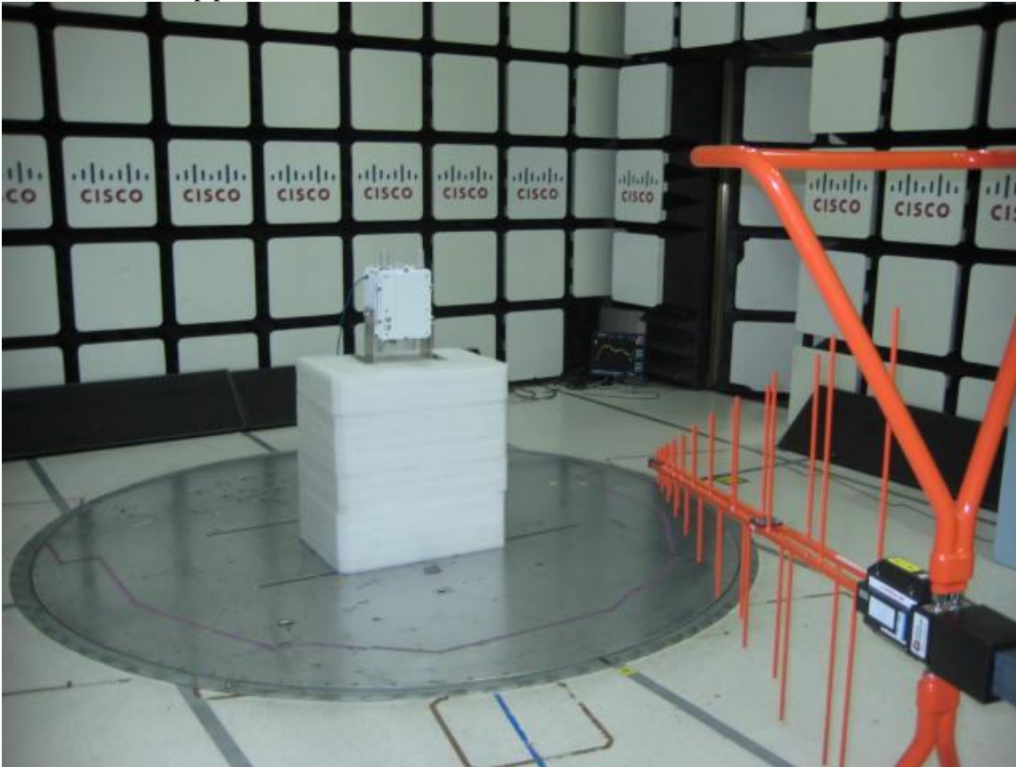
Radiated Emissions test setup for 30MHz to 1GHz in 5m chamber. Support is made of Styrofoam
