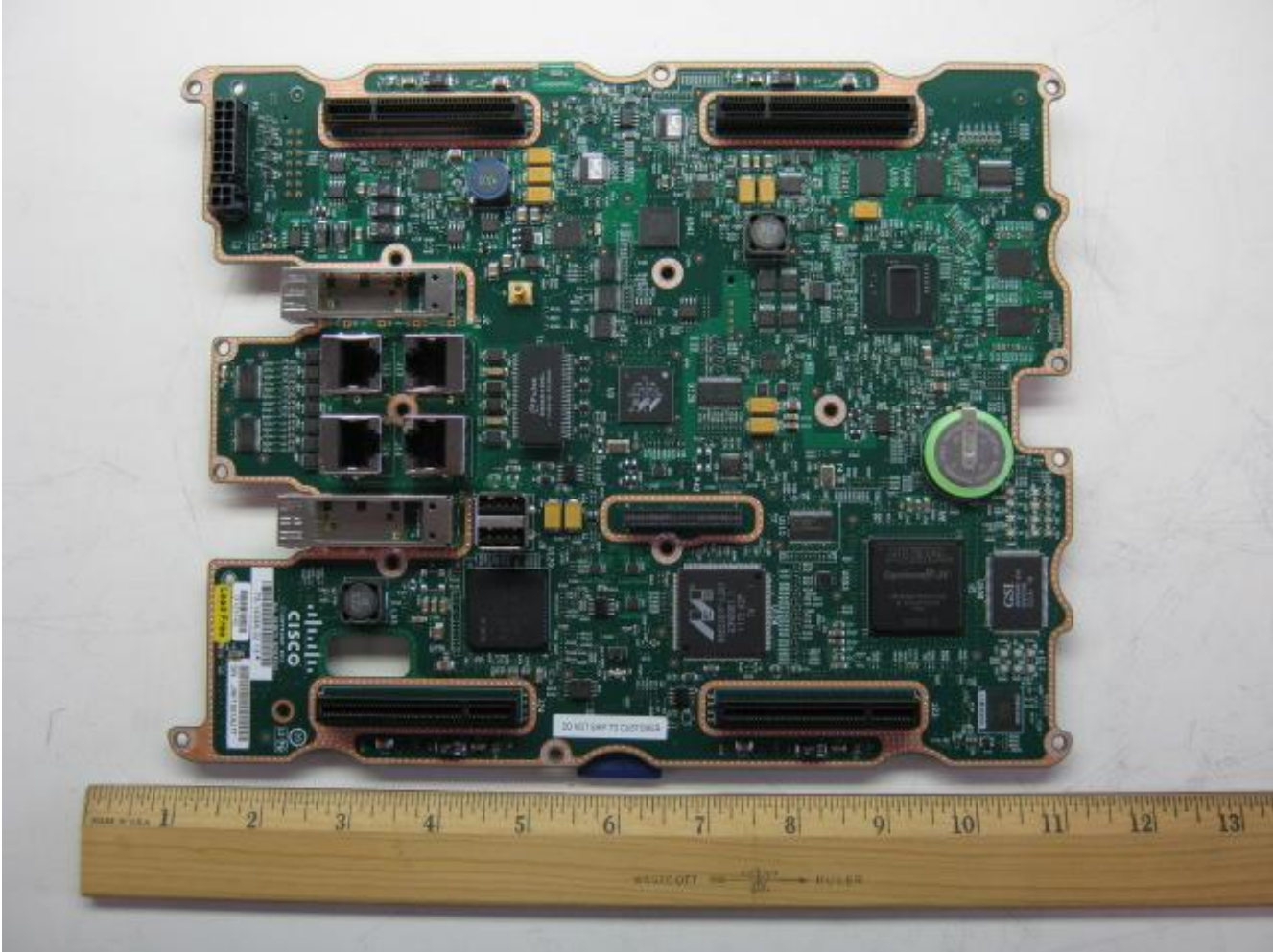
CGR1240 : Internal PCB Mother Board (Top)
