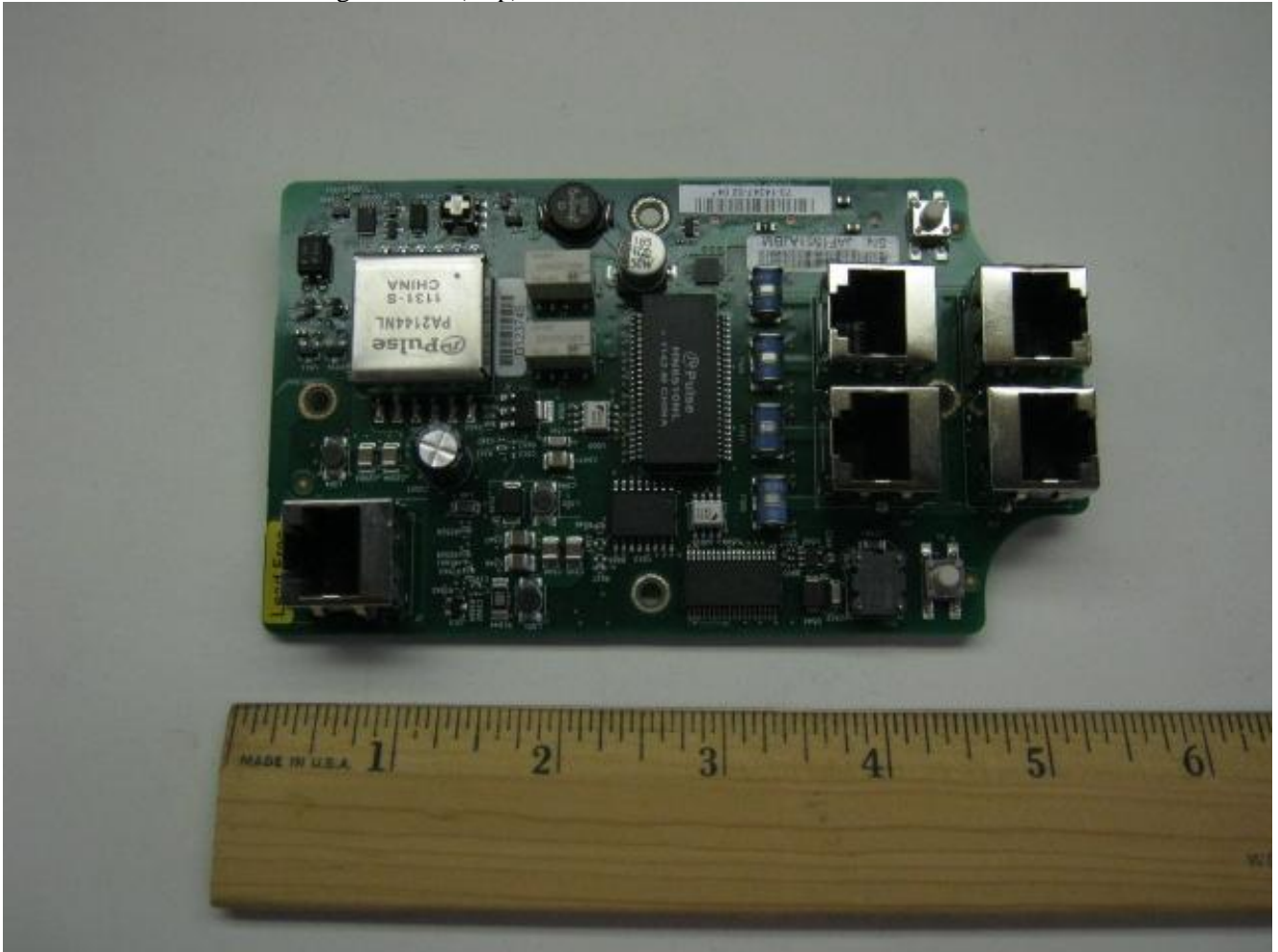
CGR1240 : Internal PCB Daughter card (Top)
