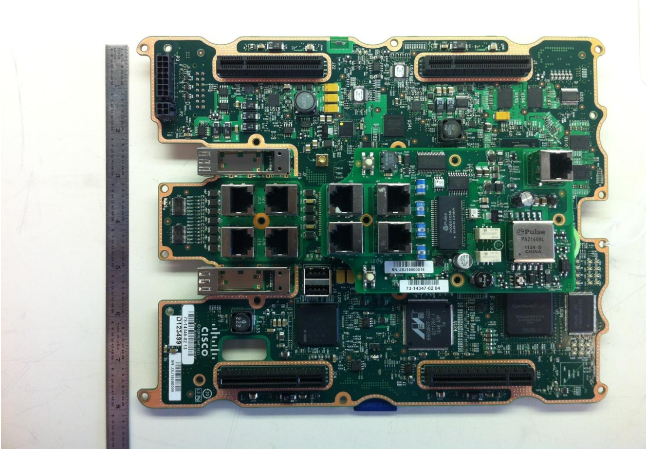
CGR-1240 : Internal PCB Mother Board (Top)
