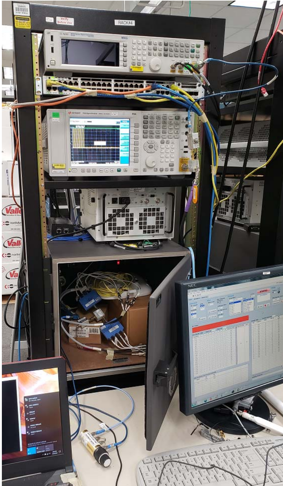
Title: Radio Conducted DFS Test Setup
