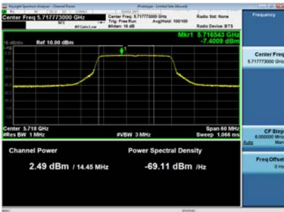
Antenna C
