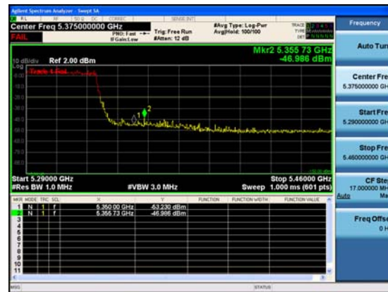
Antenna D
