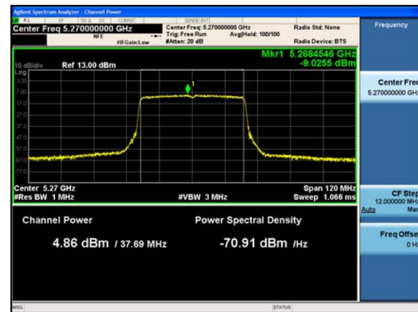
Antenna D
