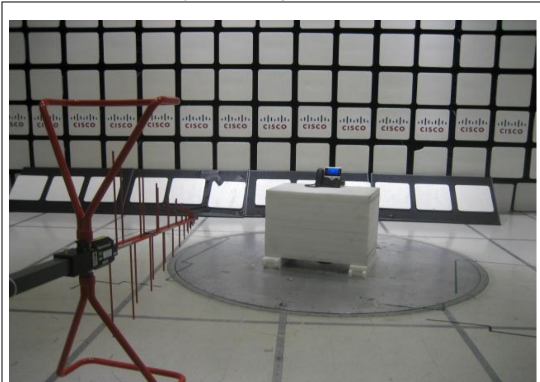
Title: Radiated Test Configuration from 30M - 1000MHz
