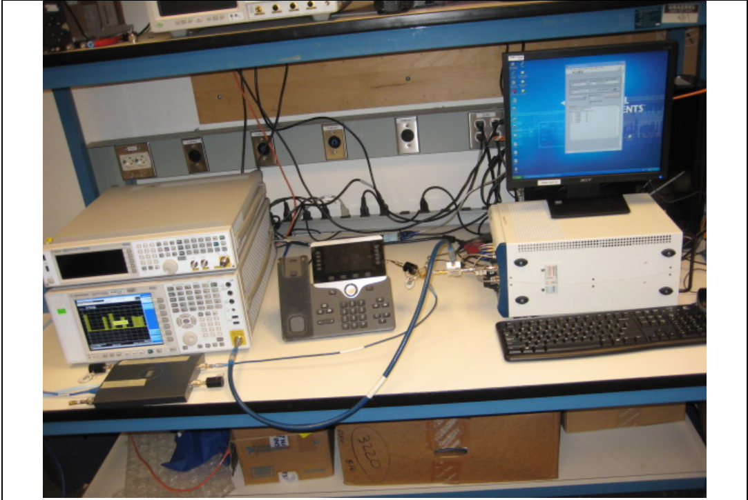
Title: DFS Test Setup
