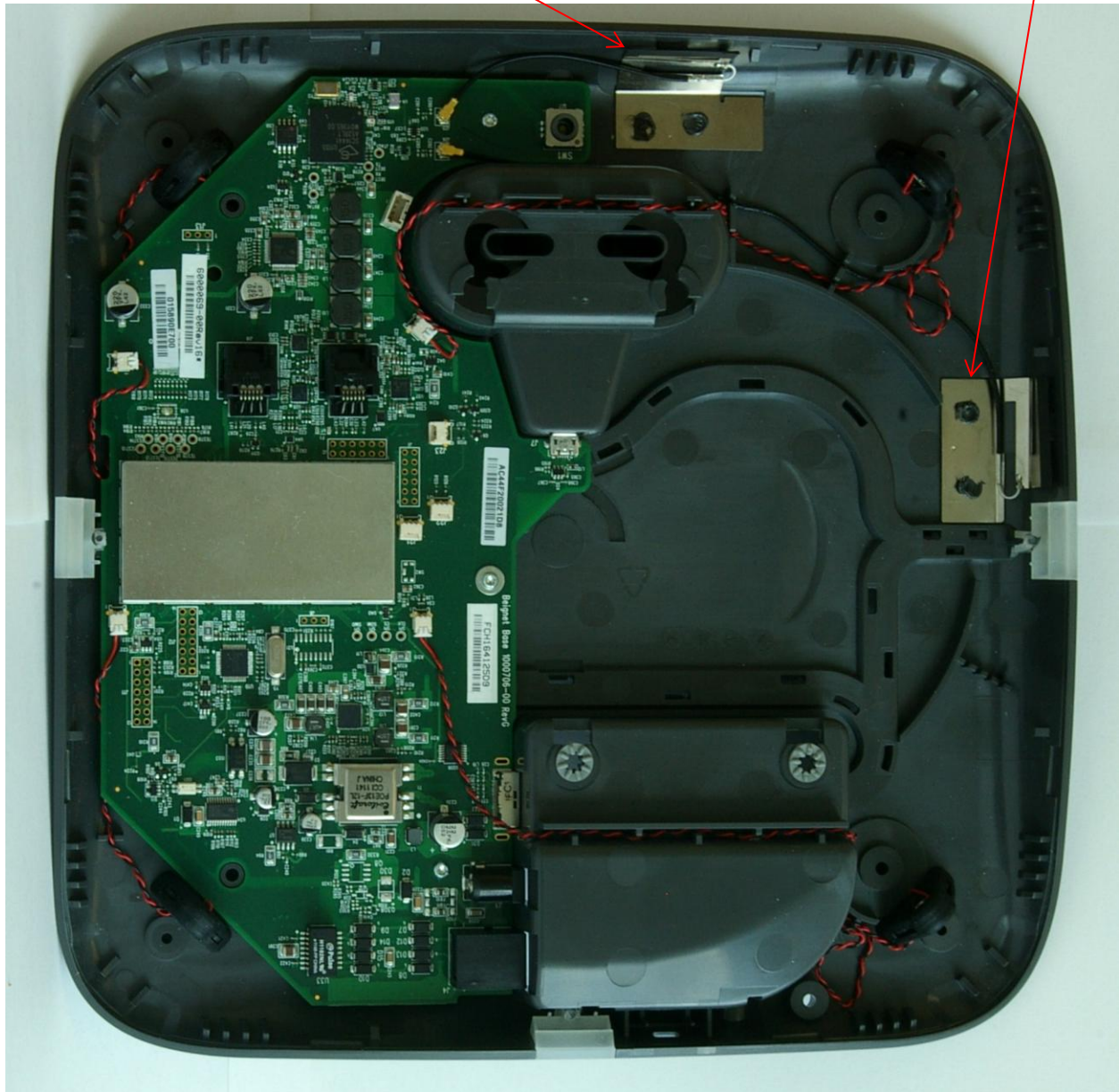
Beignet base showing antennas
