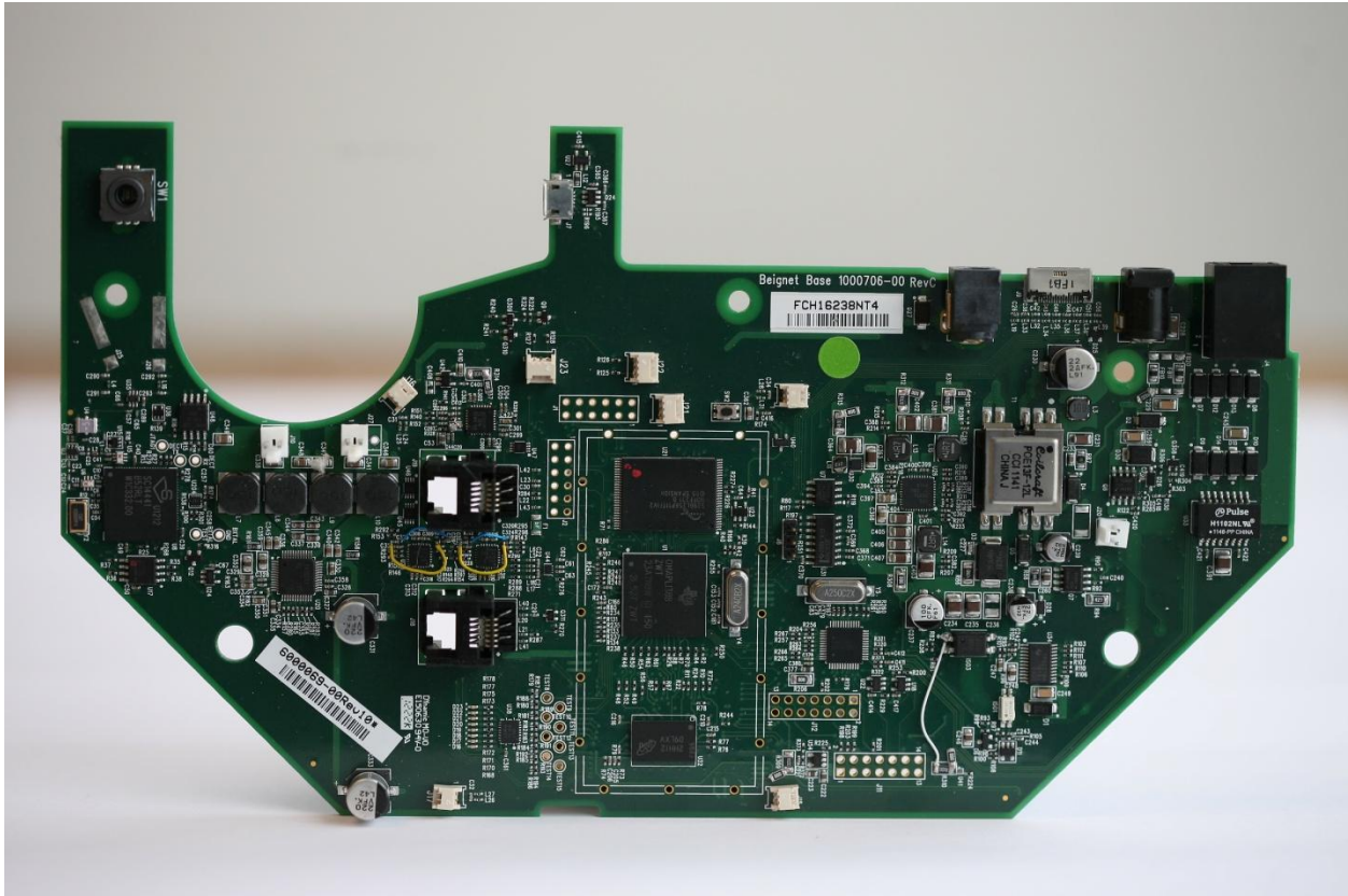
Beignet base component side
