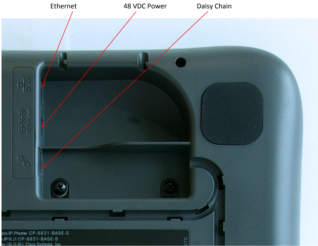
Beignet base, closeup of power and Daisy Chain port
