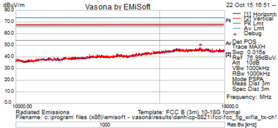
Title: TX Spurious Emissions from 10-18GHz – Ch149 (5745 MHz) – Peak Trace
