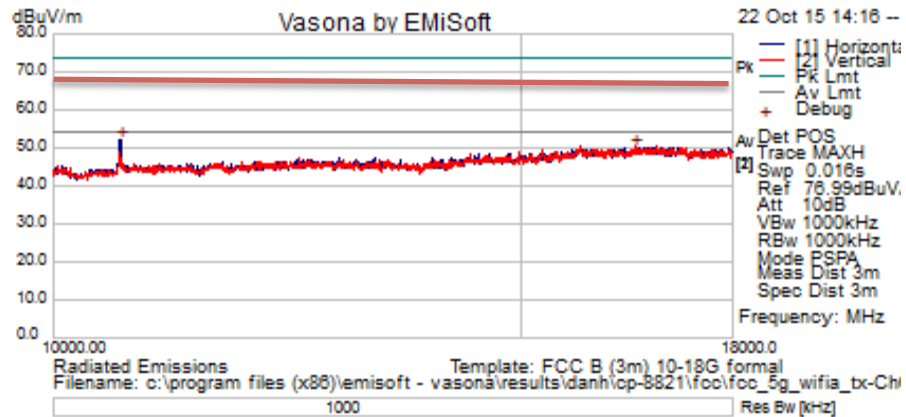
Title: TX Spurious Emissions from 10-18GHz – Ch60 (5300 MHz) – Peak Trace
