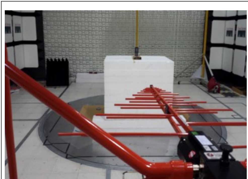
Title: Radiated Emissions Below 1 GHz
