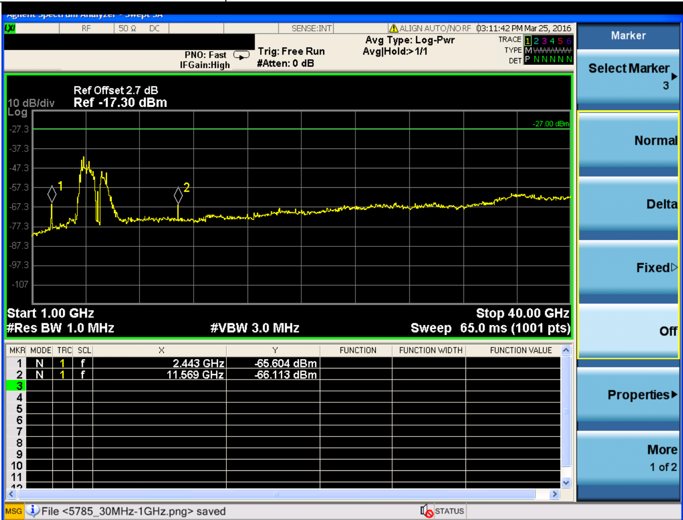
Title: TX Spurious Emissions from 1GHz-40GHz – Ch157 (5785 MHz)
