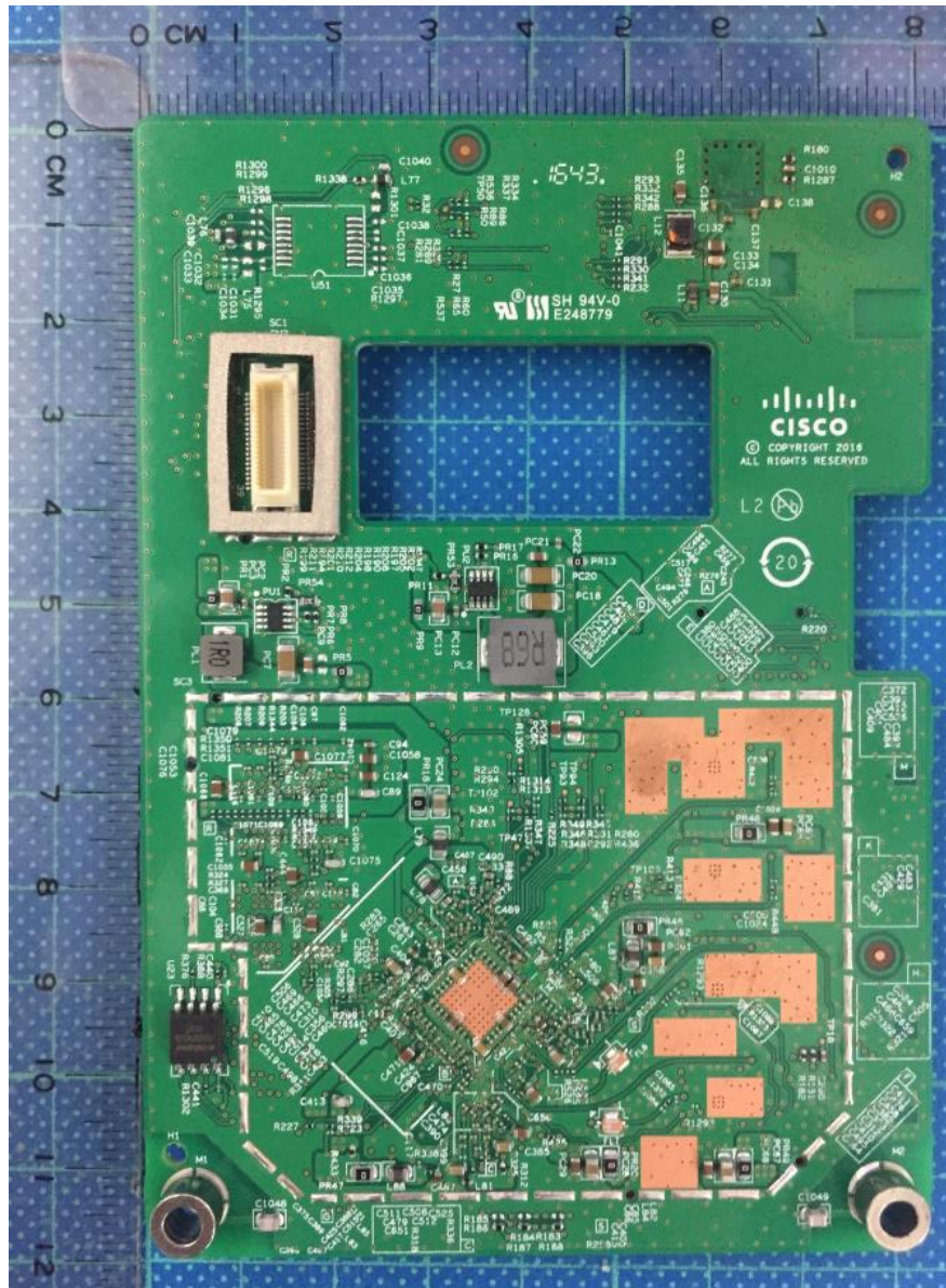
Bottom Side Board
