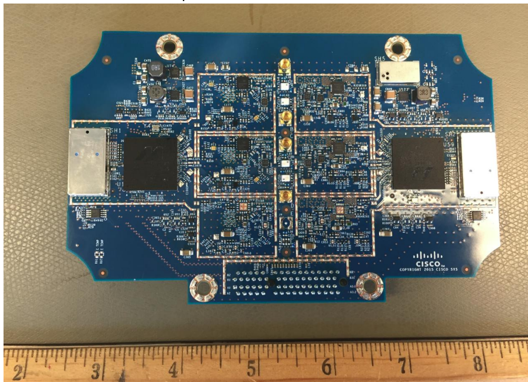
Top Side RF Board with shields
