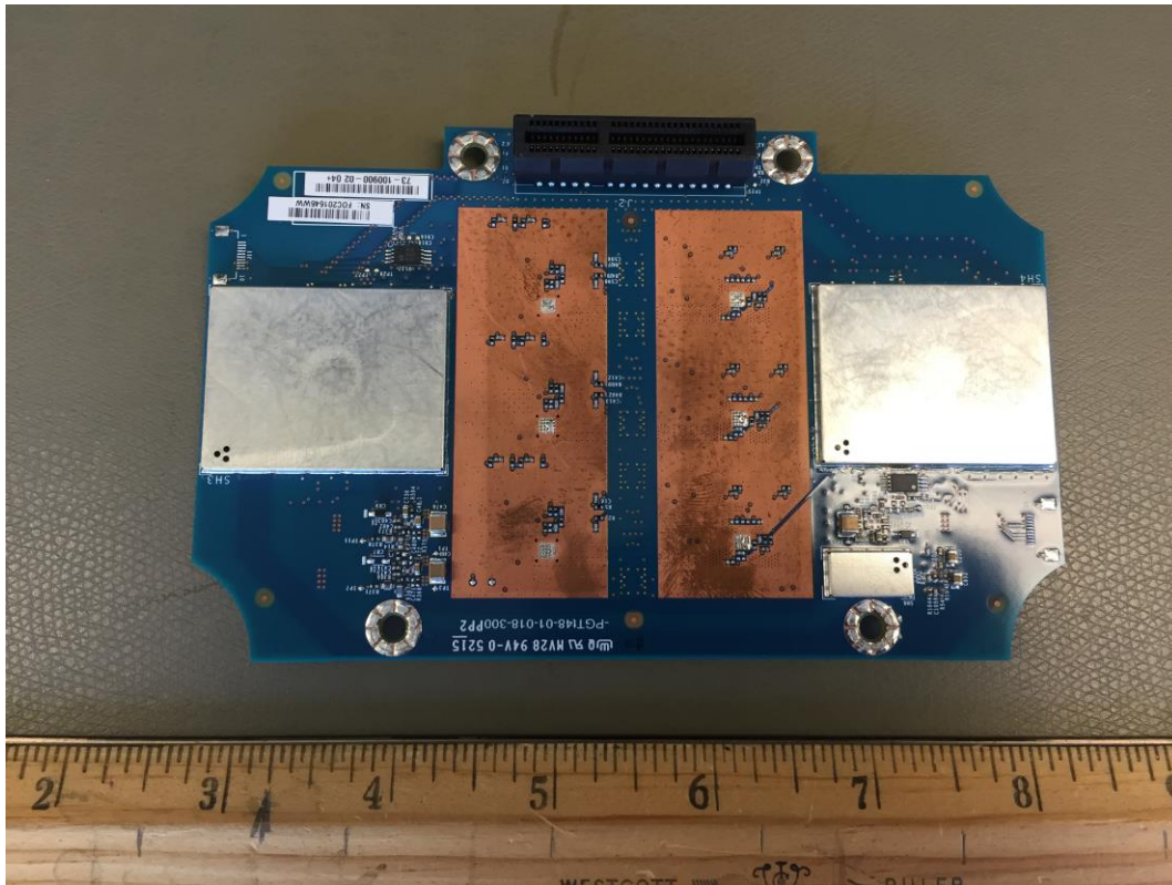
Bottom Side RF Board with Shields
