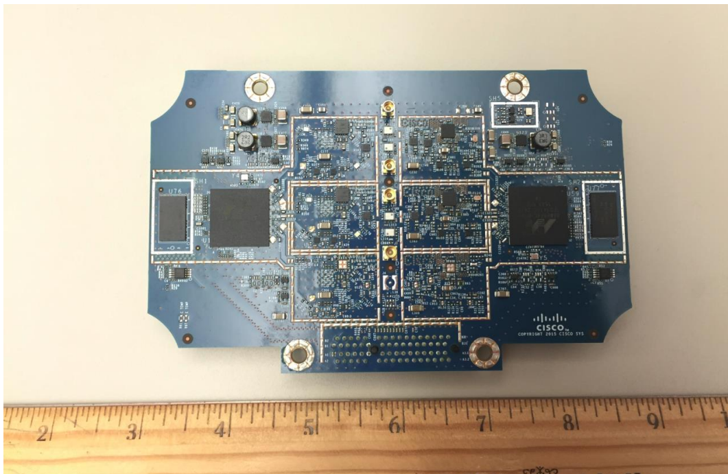
Top Side RF Board without Shields
