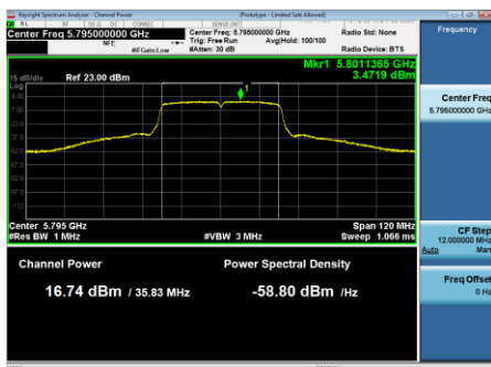
Antenna C
