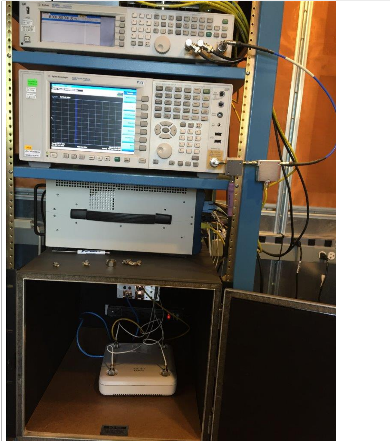
Title: Conducted Test Setup
