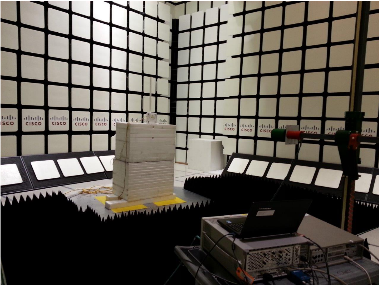
Radiated Test Setup 18GHz-40GHz
