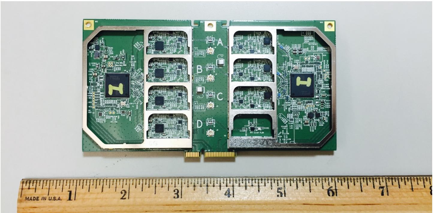
Top Side RF Board without Shields
