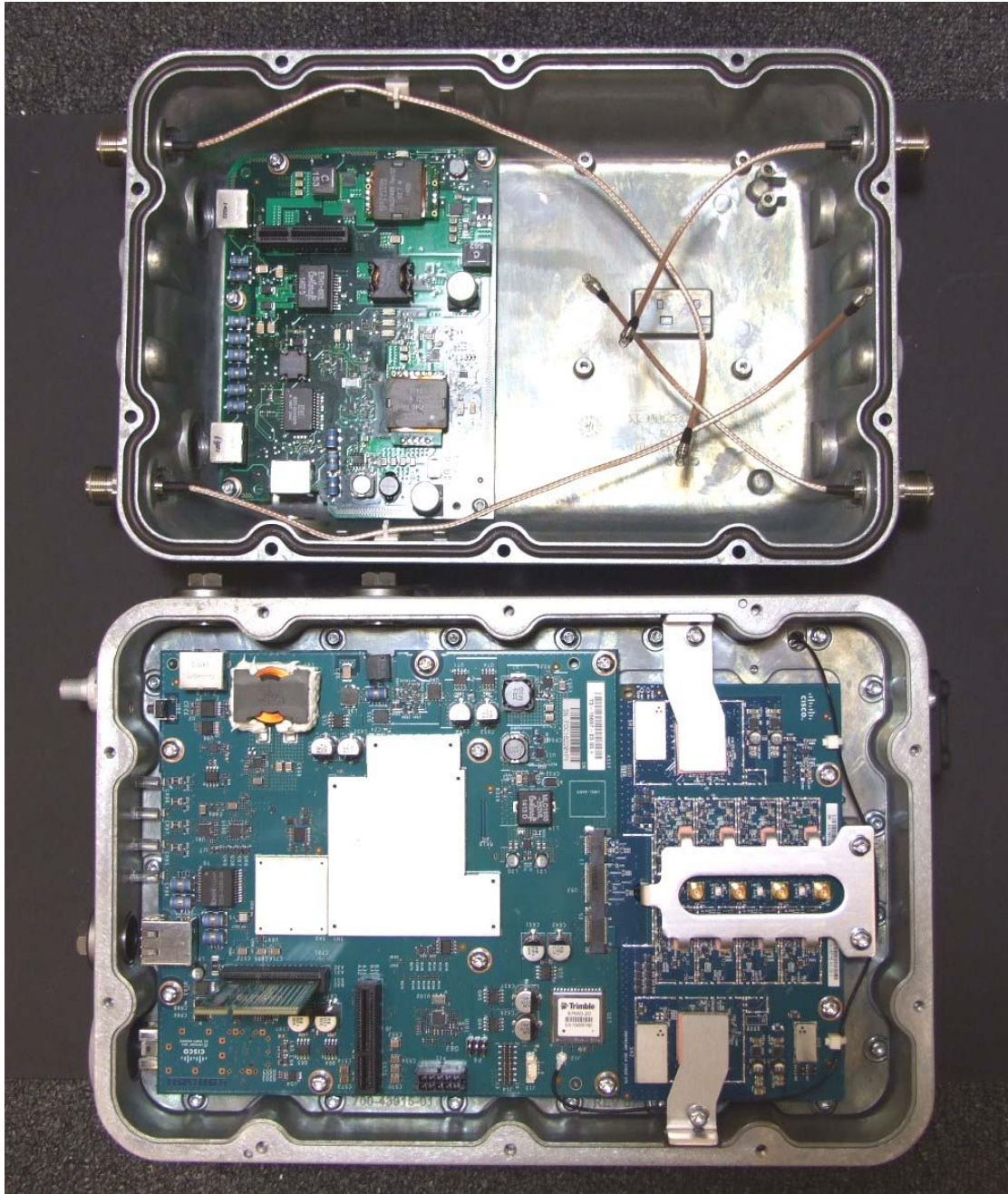
Control, Radio and PoE Supply Board
