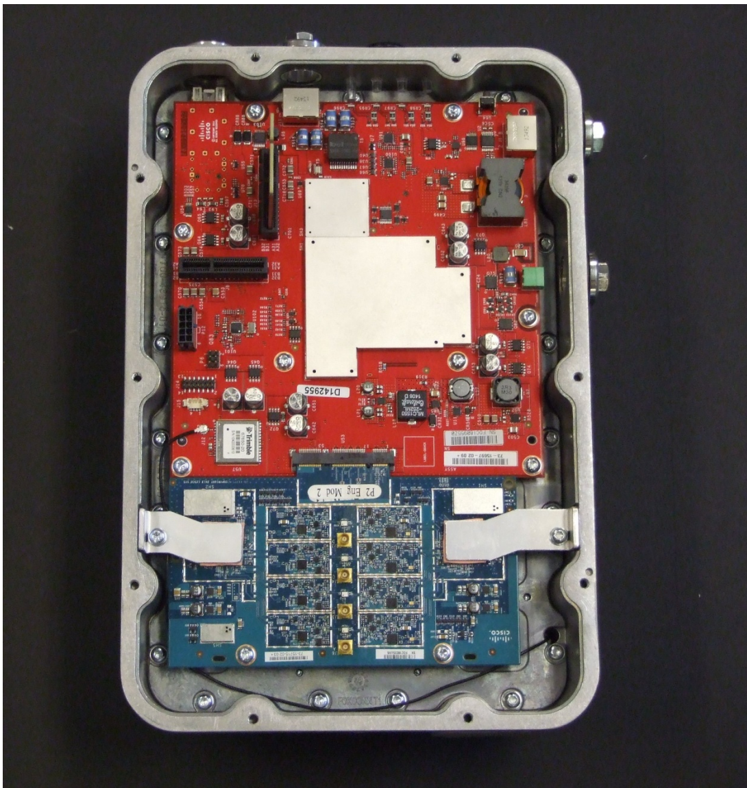
Control (red) and Radio Board
