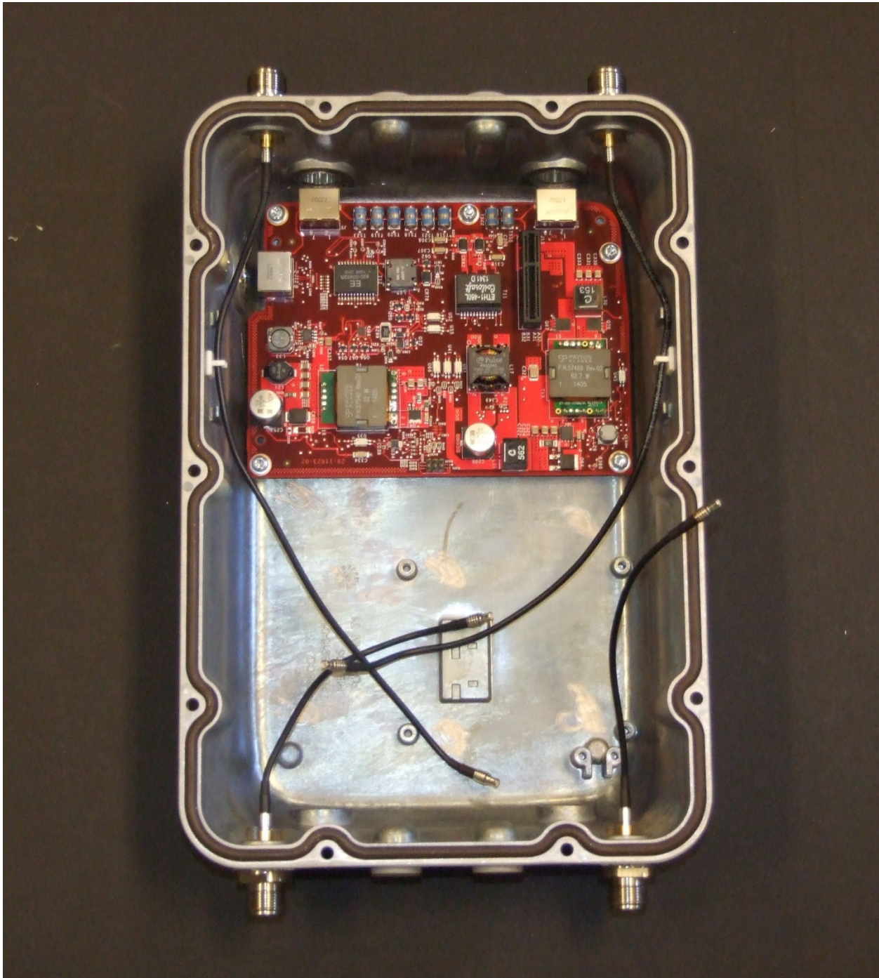
Power Over Ethernet Supply Board
