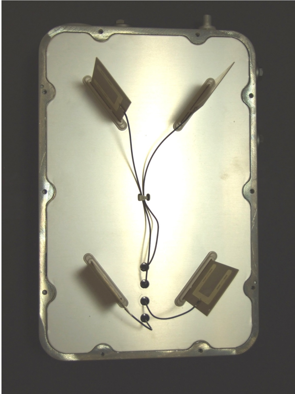
Internal Antenna Assembly
