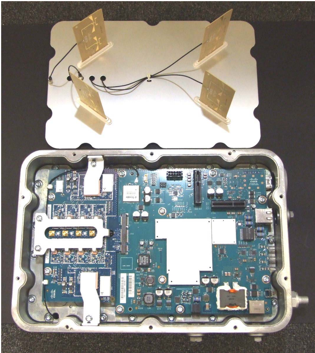
Antennas, Radio (left) and Control Boards
