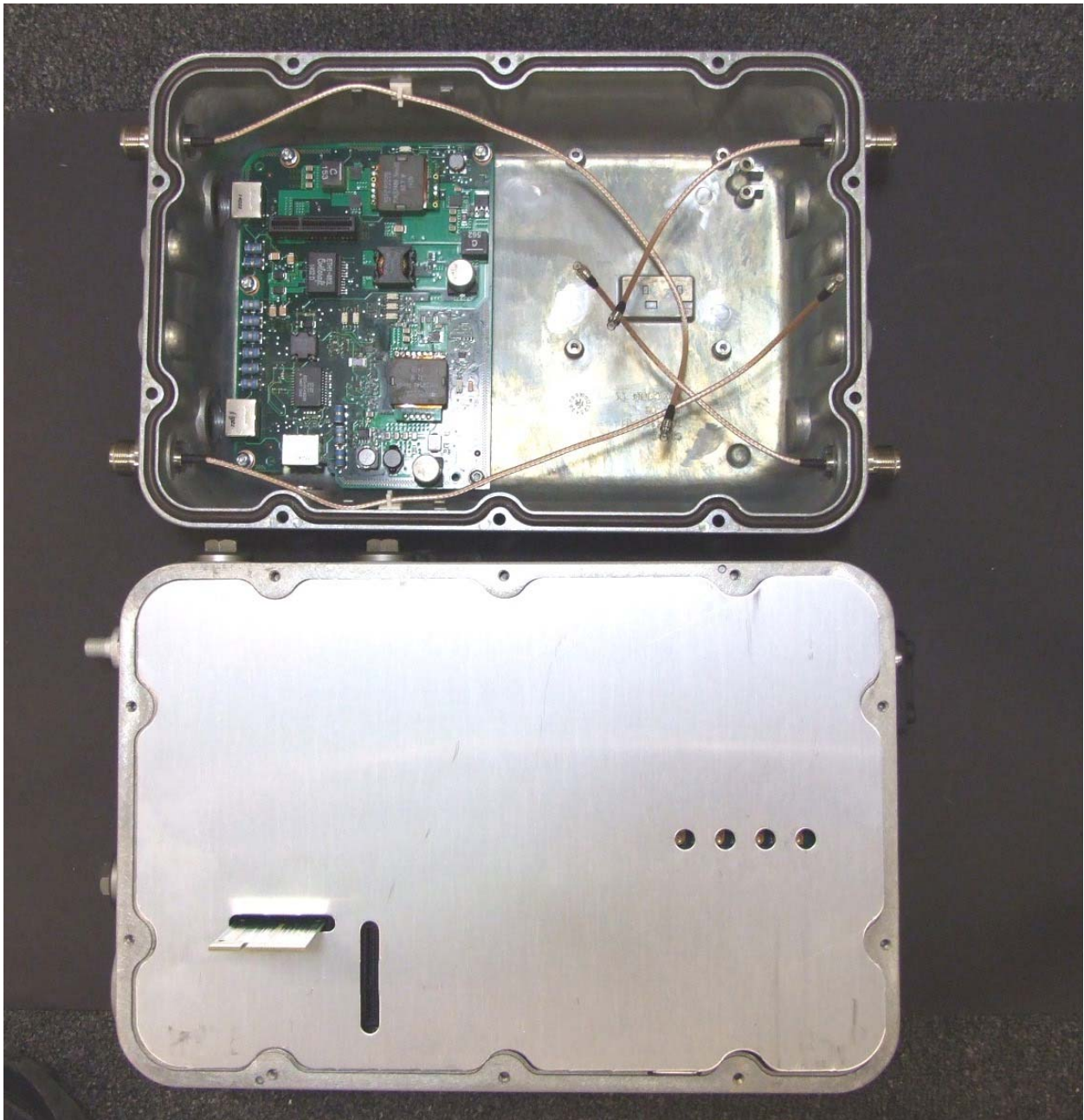
PoE Supply and internal divider
