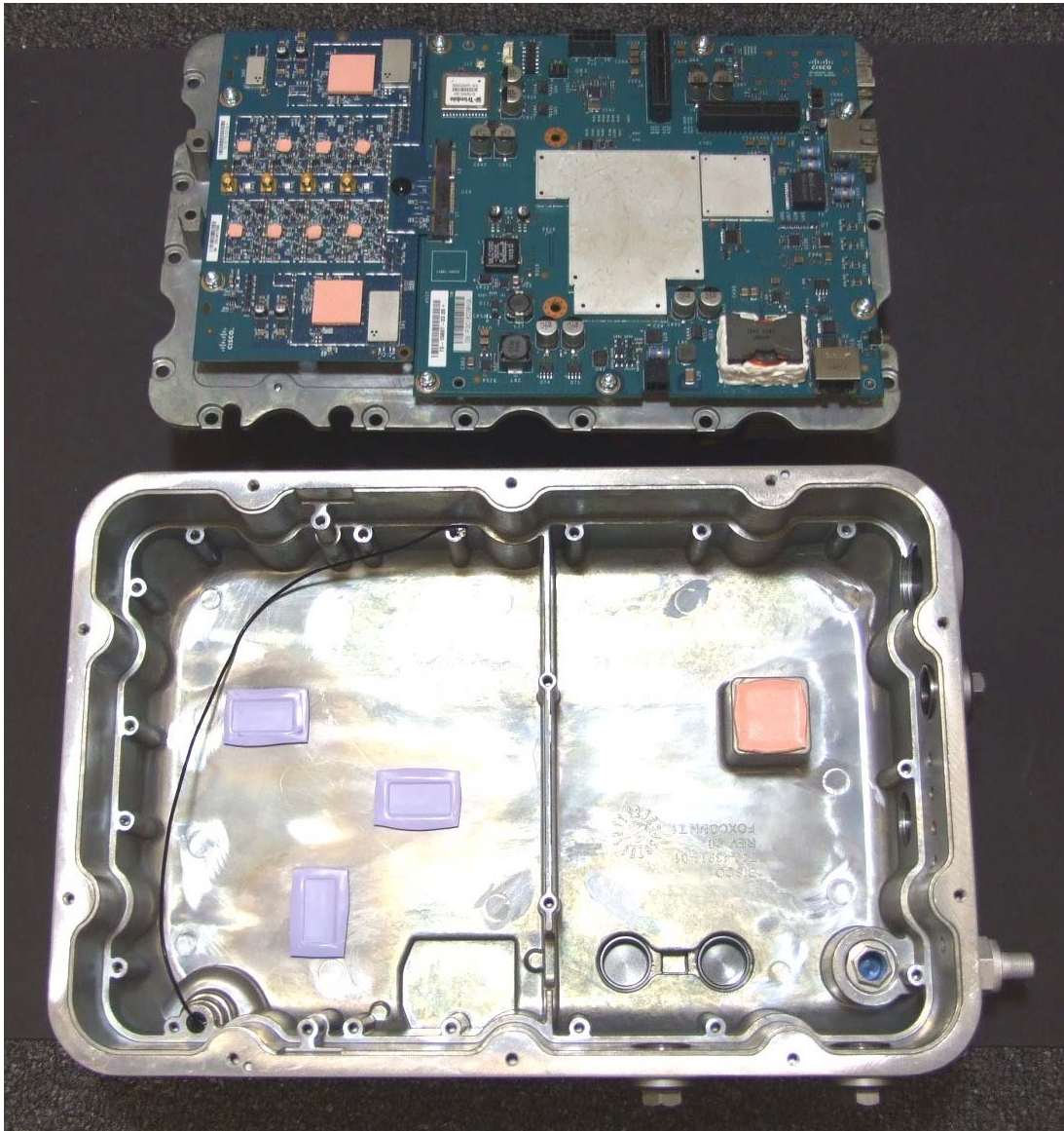
Radio, Control and Cable Connector
