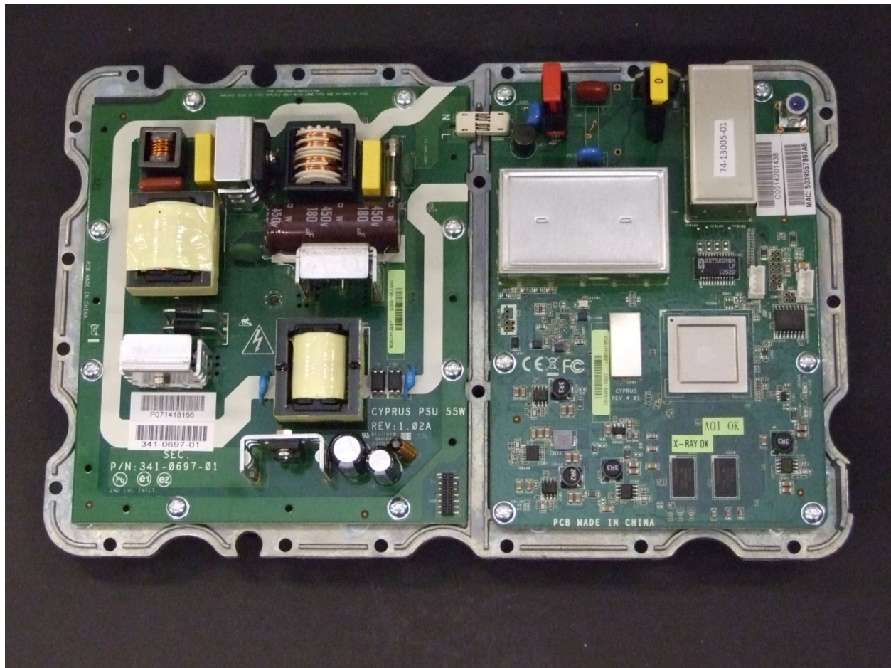
Center Panel Under Assembly
