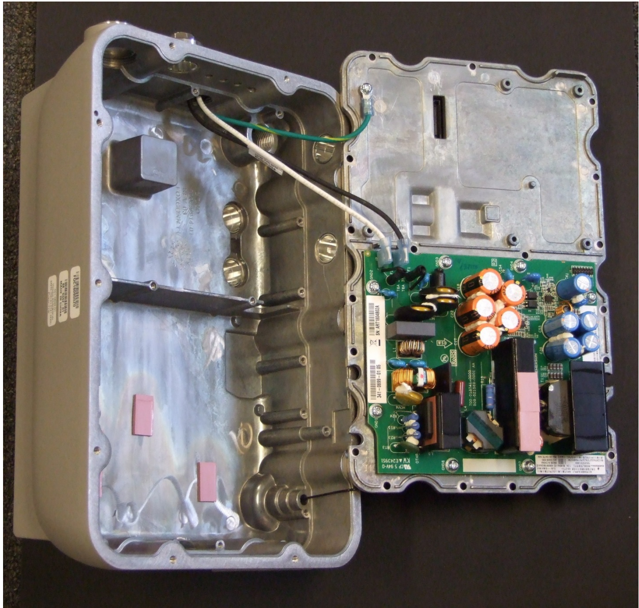
AC Power Supply
