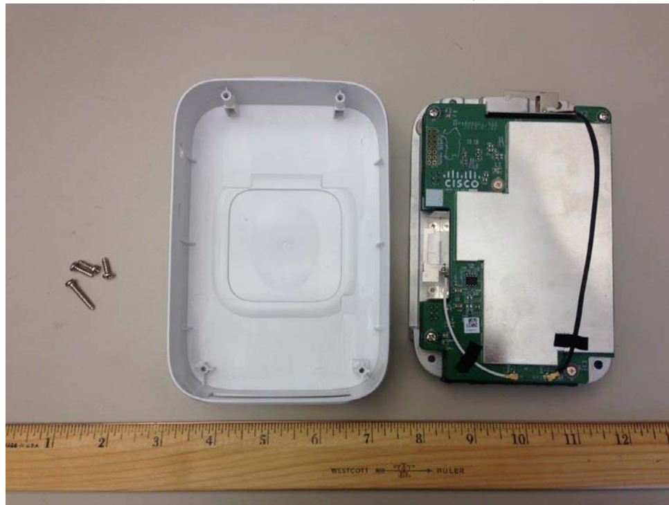
702W Series Internal Assembly
