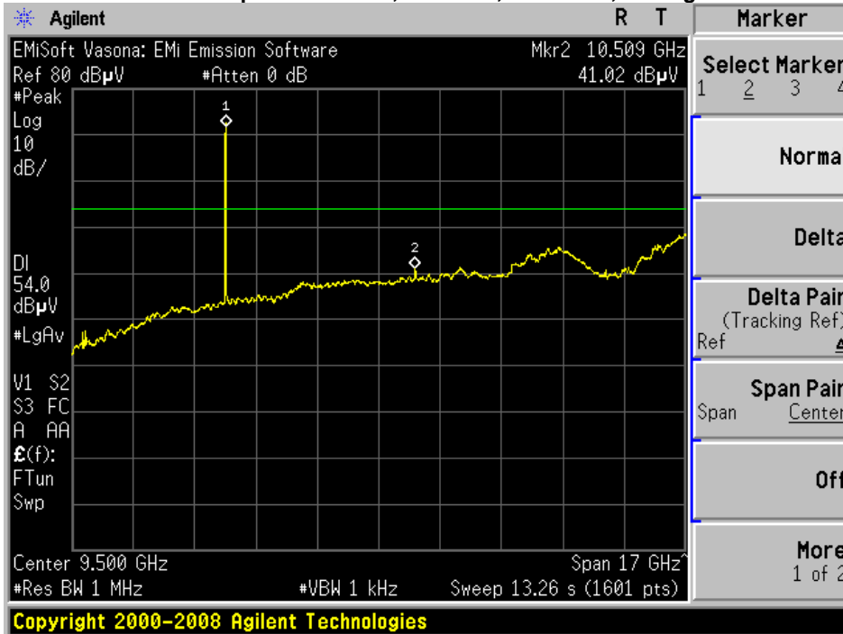
Radiated Transmitter Spurs 5260MHz, All Rates, All Modes, Average
