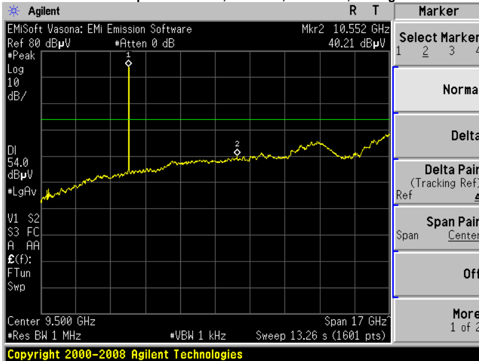
Radiated Transmitter Spurs 5280MHz, All Rates, All Modes, Average
