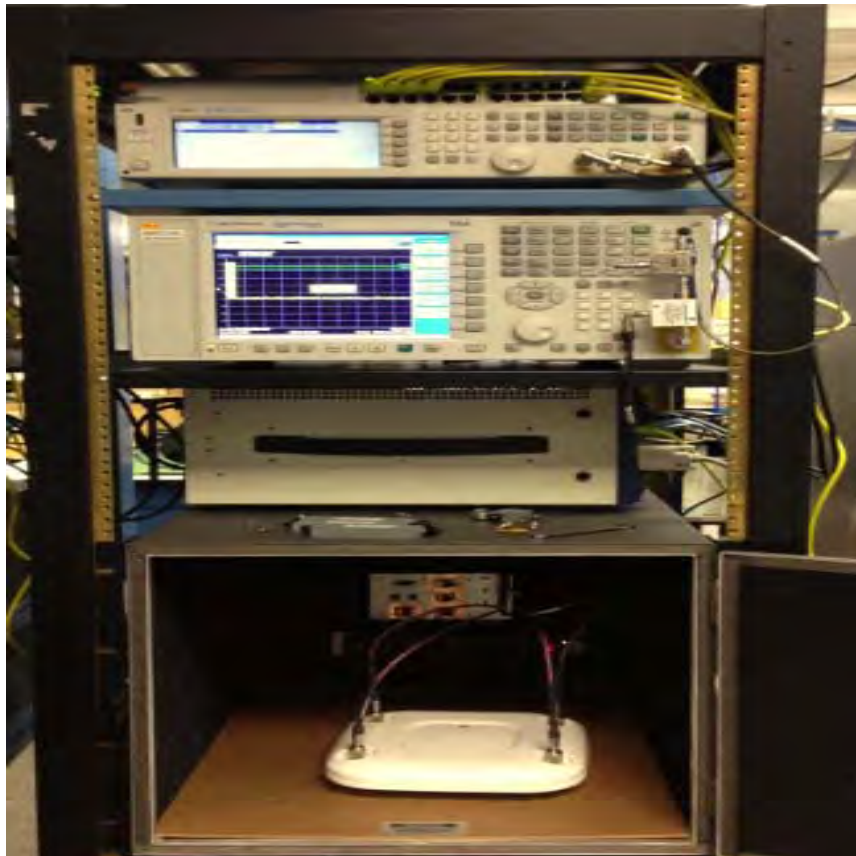
Test Setup for Conducted Measurements
