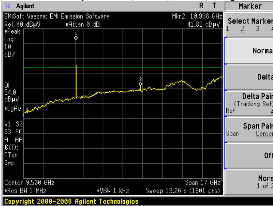
Radiated Transmitter Spurs 5500MHz, All Rates, All Modes, Average
