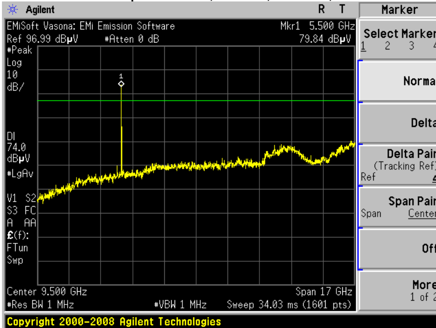
Radiated Transmitter Spurs 5500MHz, All Rates, All Modes, Peak
