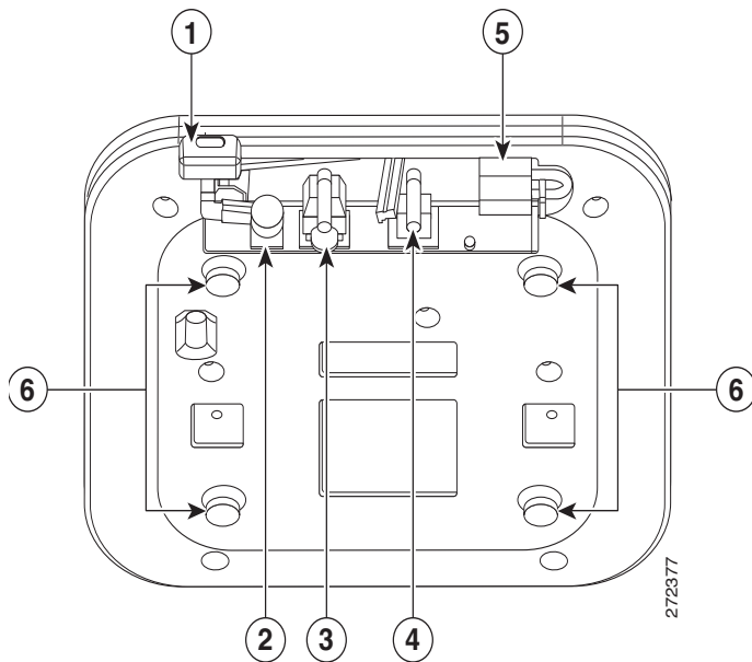
Figure 3 Access Point Ports and Connections (bottom)-AIR2702E and 2702I Models
