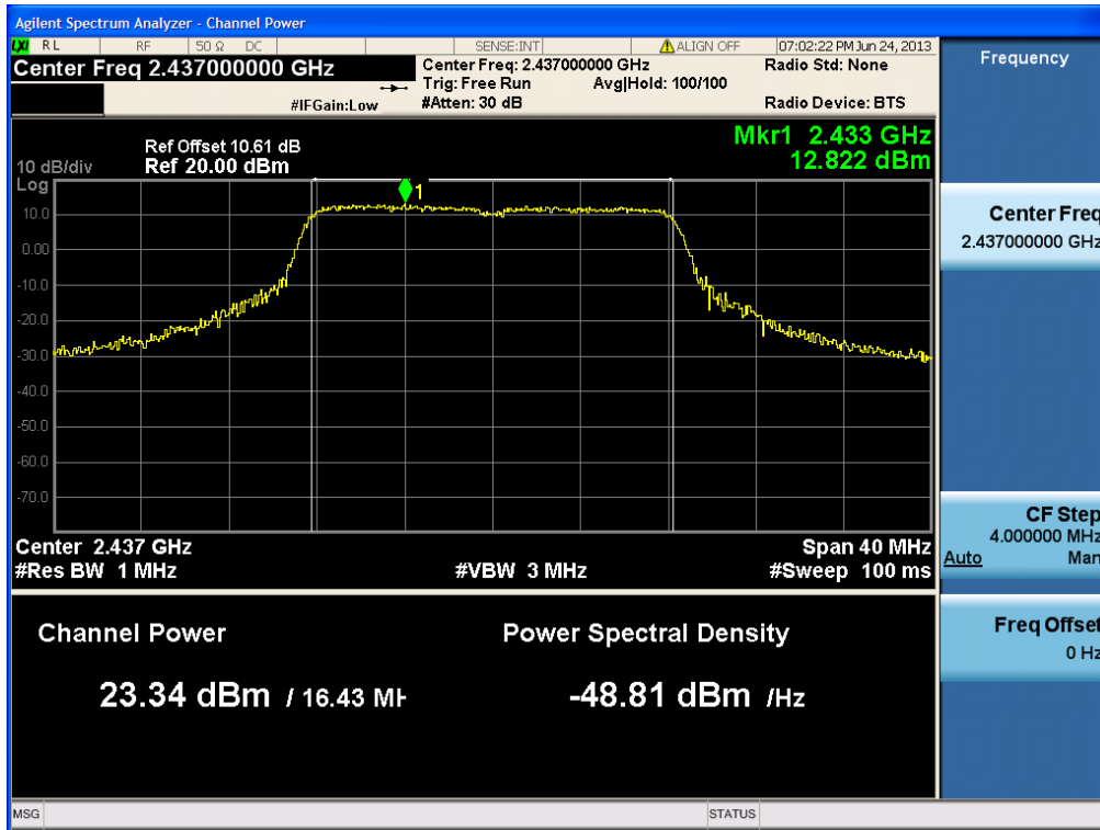
Power Spectral Density, 2437 MHz, HT-20, M0 to M23
