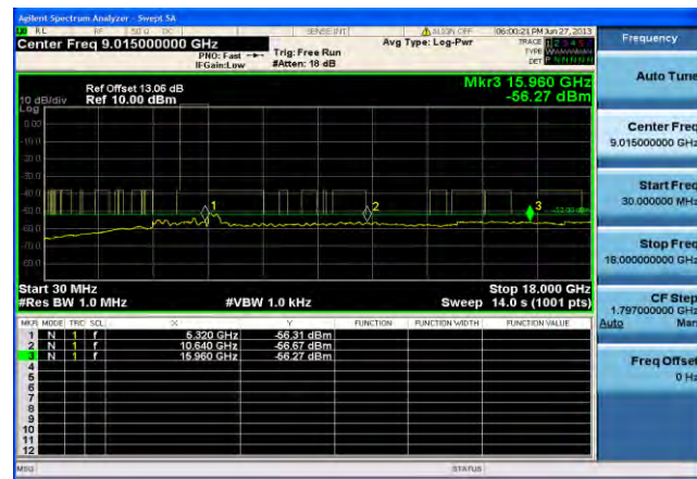
Antenna B
