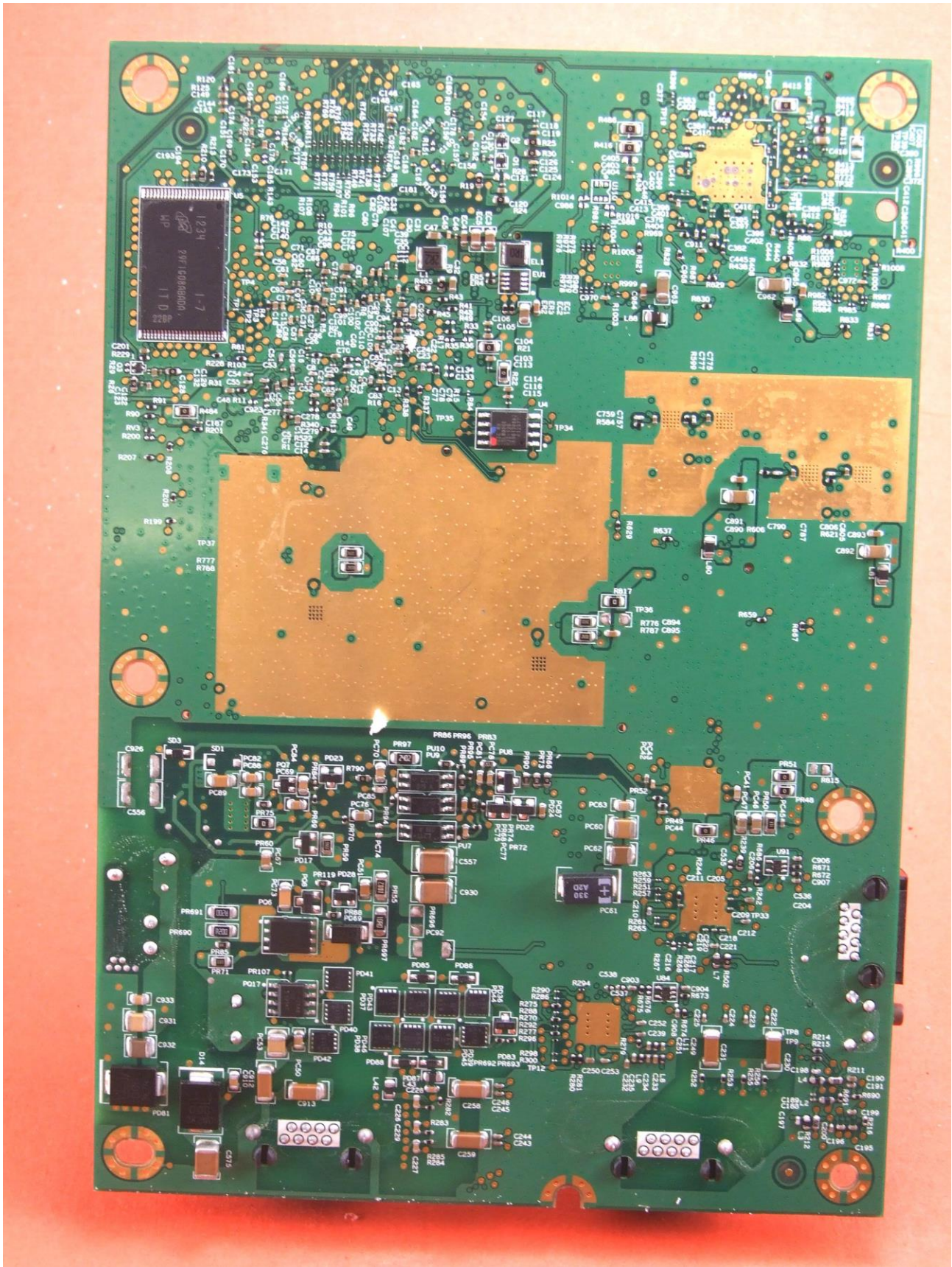
PCB – bottom
