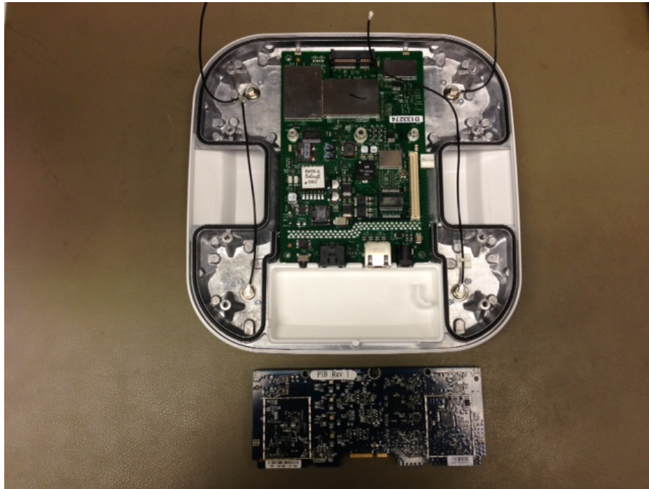
3700 Series Internal Assembly
