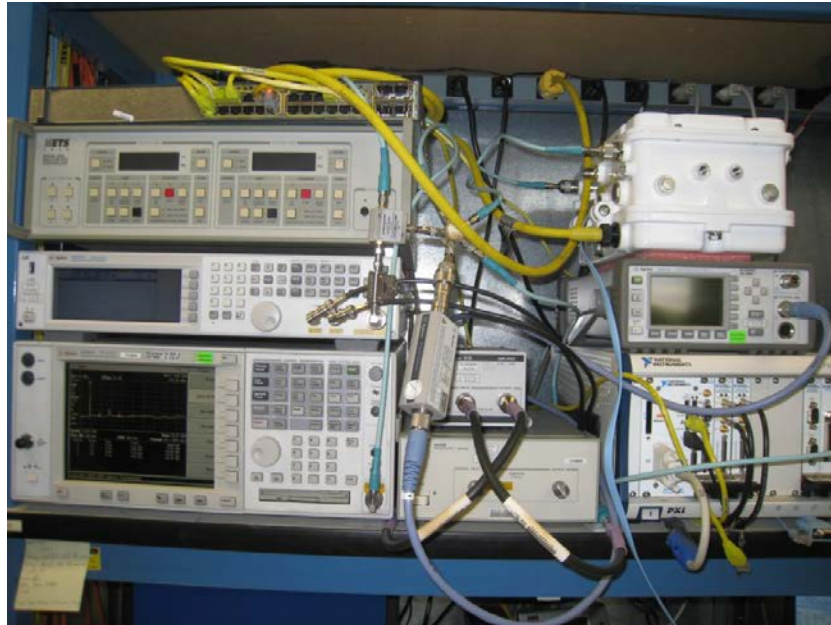
AIR-CAP1552xx Series Radiated Test Setup
